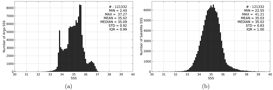
Figure 2: Histograms of SSS from Argo (a) and SMOS-L3-CATDS-IFREMER-CECOS-V2-MONTHLY-0.25DEG (b) considering all match-up pairs per bins of 0.1 over the Indian Ocean Pi-MEP region and for the full satellite product period.
