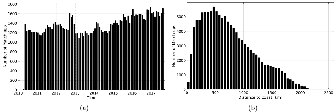
Figure 1: Number of match-ups between Argo and SMOS-L3-CATDS-IFREMER-CECOS-V2-MONTHLY-0.25DEG SSS as a function of time (a) and as function of the distance to coast (b) over the Indian Ocean Pi-MEP region and for the full satellite product period.
