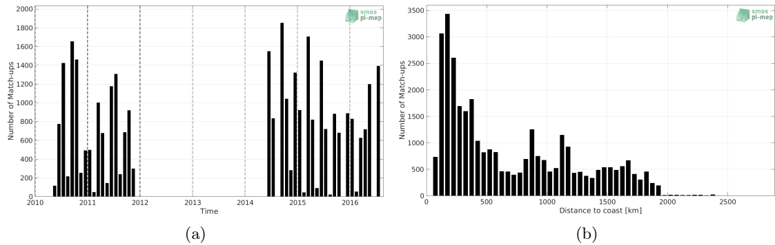
Figure 1: Number of match-ups between TSG (LEGOS-DM) and SMOS SSS L3 v2 - Daily - 0.5 Deg (CATDS-CECOS-IFREMER) SSS as a function of time (a) and as function of the distance to coast (b) over the Indian Ocean Pi-MEP region and for the full satellite product period.
