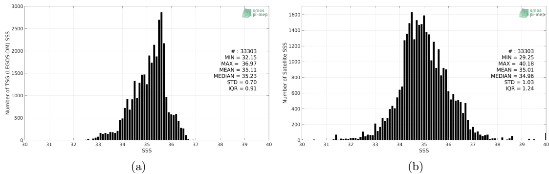
Figure 2: Histograms of SSS from TSG (LEGOS-DM) (a) and SMOS SSS L3 v2 - Daily - 0.5 Deg (CATDS-CECOS-IFREMER) (b) considering all match-up pairs per bins of 0.1 over the Indian Ocean Pi-MEP region and for the full satellite product period.
