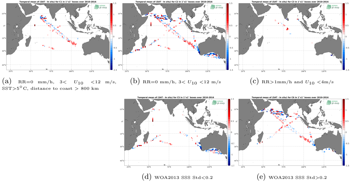
Figure 12: Temporal mean gridded over spatial boxes of size 1^{\circ}\times 1^{\circ} of \Delta\text{SSS} (SMOS SSS L3 v2 - Daily - 0.5 Deg (CATDS-CECOS-IFREMER) - TSG (LEGOS-DM)) for 5 different subdatasets corresponding to:RR=0 mm/h, 3 < U_{10} < 12 m/s, SST >5^{\circ}\text{C} , distance to coast > 800 km (a), RR=0 mm/h, 3 < U_{10} < 12 m/s (b), RR >1 mm/h and U_{10} < 4 m/s (c), WOA2013 SSS Std <0.2 (d), WOA2013 SSS Std >0.2 (e).
