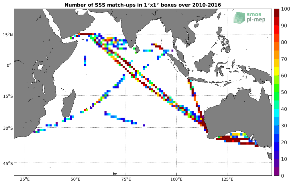
Figure 4: Number of SSS match-ups between TSG (LEGOS-DM) SSS and the SMOS SSS L3 v2 - Daily - 0.5 Deg (CATDS-CECOS-IFREMER) SSS product for the Indian Ocean Pi-MEP region over 1^\circ \times 1^\circ boxes and for the full satellite product period.
