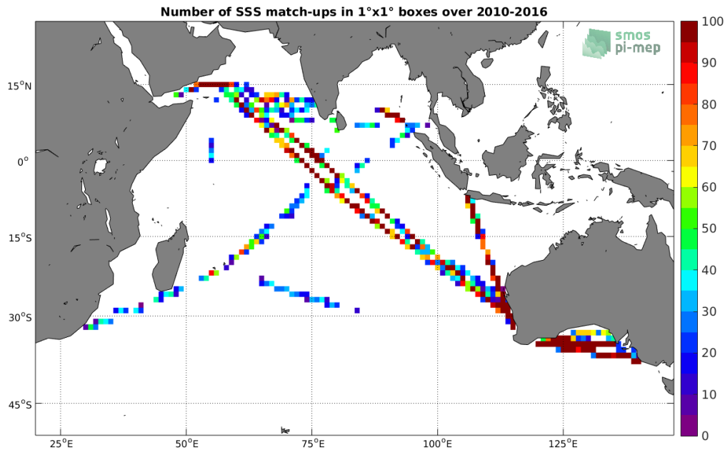
Figure 4: Number of SSS match-ups between TSG (LEGOS-DM) SSS and the SMOS SSS L3 v2 - Daily - 0.5 Deg (CATDS-CECOS-IFREMER) SSS product for the Indian Ocean Pi-MEP region over 1^\circ \times 1^\circ boxes and for the full satellite product period.
