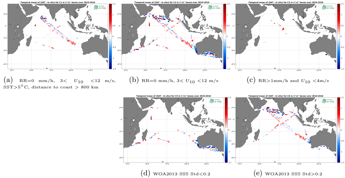
Figure 12: Temporal mean gridded over spatial boxes of size 1^{\circ}\times 1^{\circ} of \Delta\text{SSS} (SMOS L3 v2 - Daily - 0.5 Deg (CATDS-CECOS-IFREMER) - TSG-LEGOS-DM) for 5 different subdatasets corresponding to:RR=0 mm/h, 3 < U_{10} < 12 m/s, SST >5^{\circ}\text{C} , distance to coast > 800 km (a), RR=0 mm/h, 3 < U_{10} < 12 m/s (b), RR >1 mm/h and U_{10} < 4 m/s (c), WOA2013 SSS Std <0.2 (d), WOA2013 SSS Std >0.2 (e).
