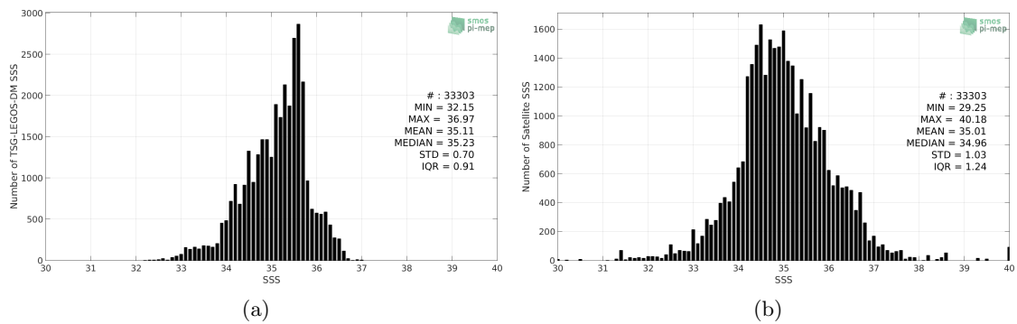
Figure 2: Histograms of SSS from TSG-LEGOS-DM (a) and SMOS L3 v2 - Daily - 0.5 Deg (CATDS-CECOS-IFREMER) (b) considering all match-up pairs per bins of 0.1 over the Indian Ocean Pi-MEP region and for the full satellite product period.
