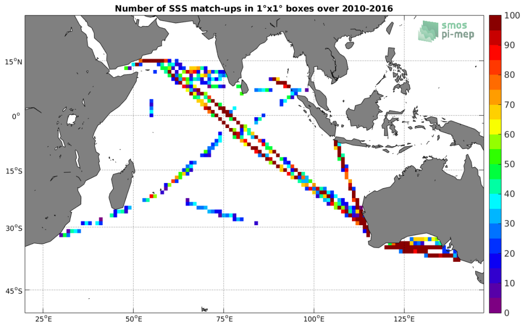
Figure 4: Number of SSS match-ups between TSG-LEGOS-DM SSS and the SMOS L3 v2 - Daily - 0.5 Deg (CATDS-CECOS-IFREMER) SSS product for the Indian Ocean Pi-MEP region over 1°x1° boxes and for the full satellite product period.
