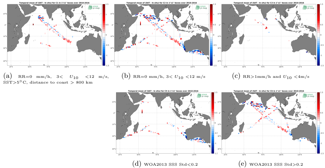
Figure 12: Temporal mean gridded over spatial boxes of size 1°x1° of \Delta SSS (SMOS-L3-CATDS-CECOS-IFREMER-V2-1DAY-0.5DEG - TSG-LEGOS-DM) for 5 different subdatasets corresponding to:RR=0 mm/h, 3 < U_{10} < 12 m/s, SST>5°C, distance to coast > 800 km (a), RR=0 mm/h, 3 < U_{10} < 12 m/s (b), RR>1mm/h and U_{10} < 4 m/s (c), WOA2013 SSS Std<0.2 (d), WOA2013 SSS Std>0.2 (e).
