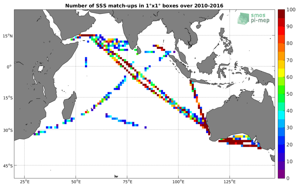
Figure 4: Number of SSS match-ups between TSG-LEGOS-DM SSS and the SMOS-L3-CATDS-CECOS-IFREMER-V2-1DAY-0.5DEG SSS product for the Indian Ocean Pi-MEP region over 1°x1° boxes and for the full satellite product period.
