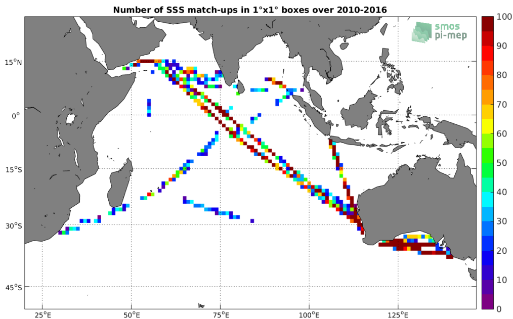
Figure 4: Number of SSS match-ups between TSG-LEGOS-DM SSS and the SMOS-L3-CATDS-CECOS-IFREMER-V2-1DAY-0.5DEG SSS product for the Indian Ocean Pi-MEP region over 1^\circ \times 1^\circ boxes and for the full satellite product period.
