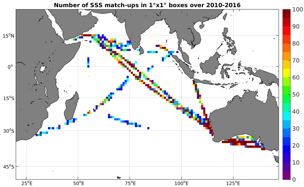
Figure 4: Number of SSS match-ups between TSG-LEGOS-DM SSS and the SMOS-L3-CATDS-CECOS-IFREMER-V2-1DAY-0.5DEG SSS product for the Indian Ocean Pi-MEP region over 1^{\circ} \times 1^{\circ} boxes and for the full satellite product period.
