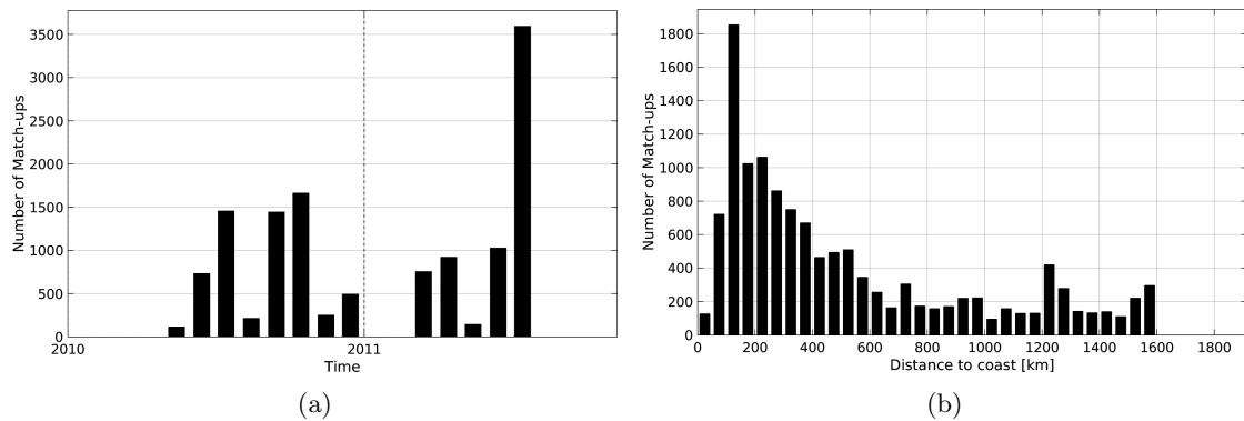
Figure 1: Number of match-ups between TSG-LEGOS-DM and SMOS-L3-CATDS-CECOS-IFREMER-V2-1DAY-0.5deg SSS as a function of time (a) and as function of the distance to coast (b) over the Indian Ocean Pi-MEP region and for the full satellite product period.
