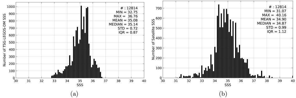
Figure 2: Histograms of SSS from TSG-LEGOS-DM (a) and SMOS-L3-CATDS-CECOS-IFREMER-V2-1DAY-0.5deg (b) considering all match-up pairs per bins of 0.1 over the Indian Ocean Pi-MEP region and for the full satellite product period.
