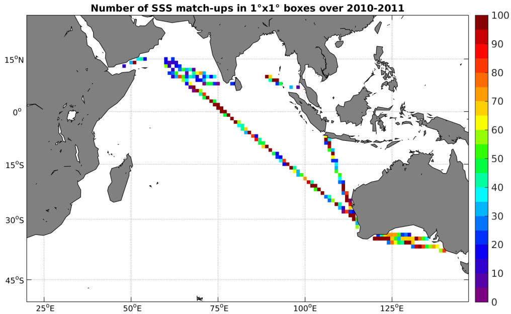
Figure 4: Number of SSS match-ups between TSG-LEGOS-DM SSS and the SMOS-L3-CATDS-CECOS-IFREMER-V2-1DAY-0.5deg SSS product for the Indian Ocean Pi-MEP region over 1°x1° boxes and for the full satellite product period.
