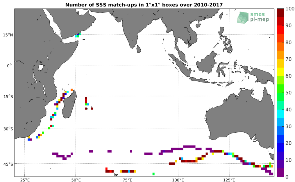
Figure 4: Number of SSS match-ups between TSG (GOSUD-Sailing-ship) SSS and the SMOS SSS L3 v2 - Daily - 0.5 Deg (CATDS-CECOS-IFREMER) SSS product for the Indian Ocean Pi-MEP region over 1^\circ \times 1^\circ boxes and for the full satellite product period.
