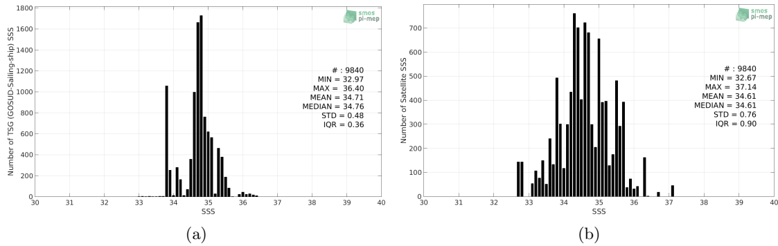
Figure 2: Histograms of SSS from TSG (GOSUD-Sailing-ship) (a) and SMOS SSS L3 v2 - Daily - 0.5 Deg (CATDS-CECOS-IFREMER) (b) considering all match-up pairs per bins of 0.1 over the Indian Ocean Pi-MEP region and for the full satellite product period.
