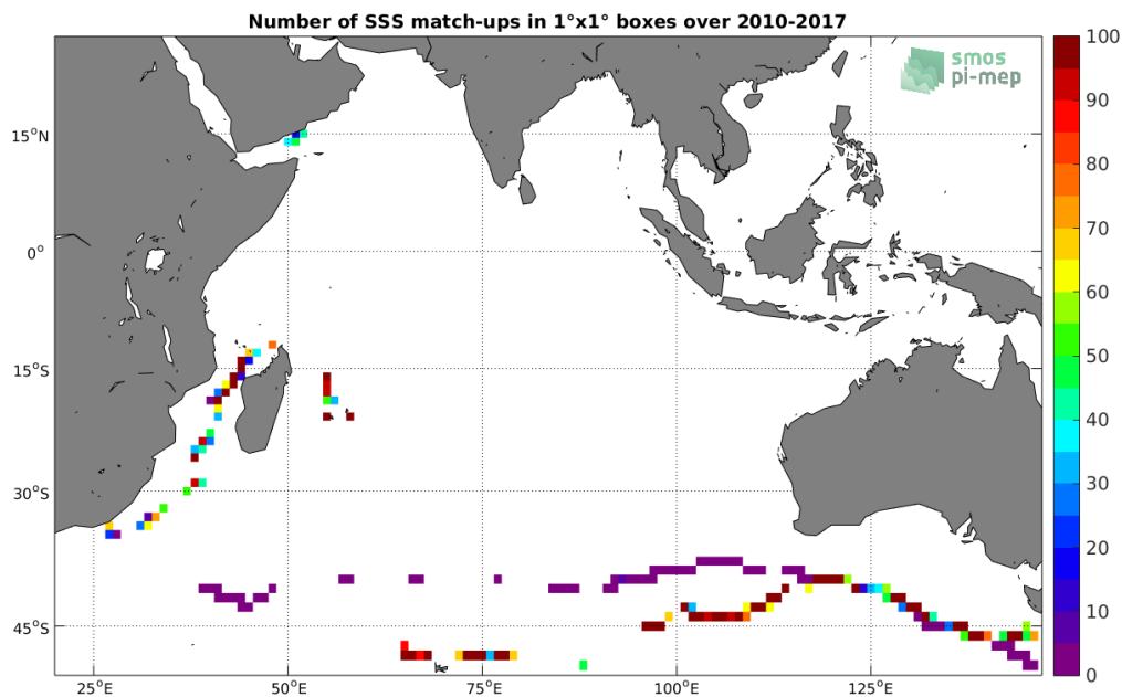
Figure 4: Number of SSS match-ups between TSG-GOSUD-Sailing-ship SSS and the SMOS L3 v2 - Daily - 0.5 Deg (CATDS-CECOS-IFREMER) SSS product for the Indian Ocean Pi-MEP region over 1°x1° boxes and for the full satellite product period.
