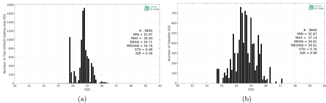
Figure 2: Histograms of SSS from TSG-GOSUD-Sailing-ship (a) and SMOS L3 v2 - Daily - 0.5 Deg (CATDS-CECOS-IFREMER) (b) considering all match-up pairs per bins of 0.1 over the Indian Ocean Pi-MEP region and for the full satellite product period.
