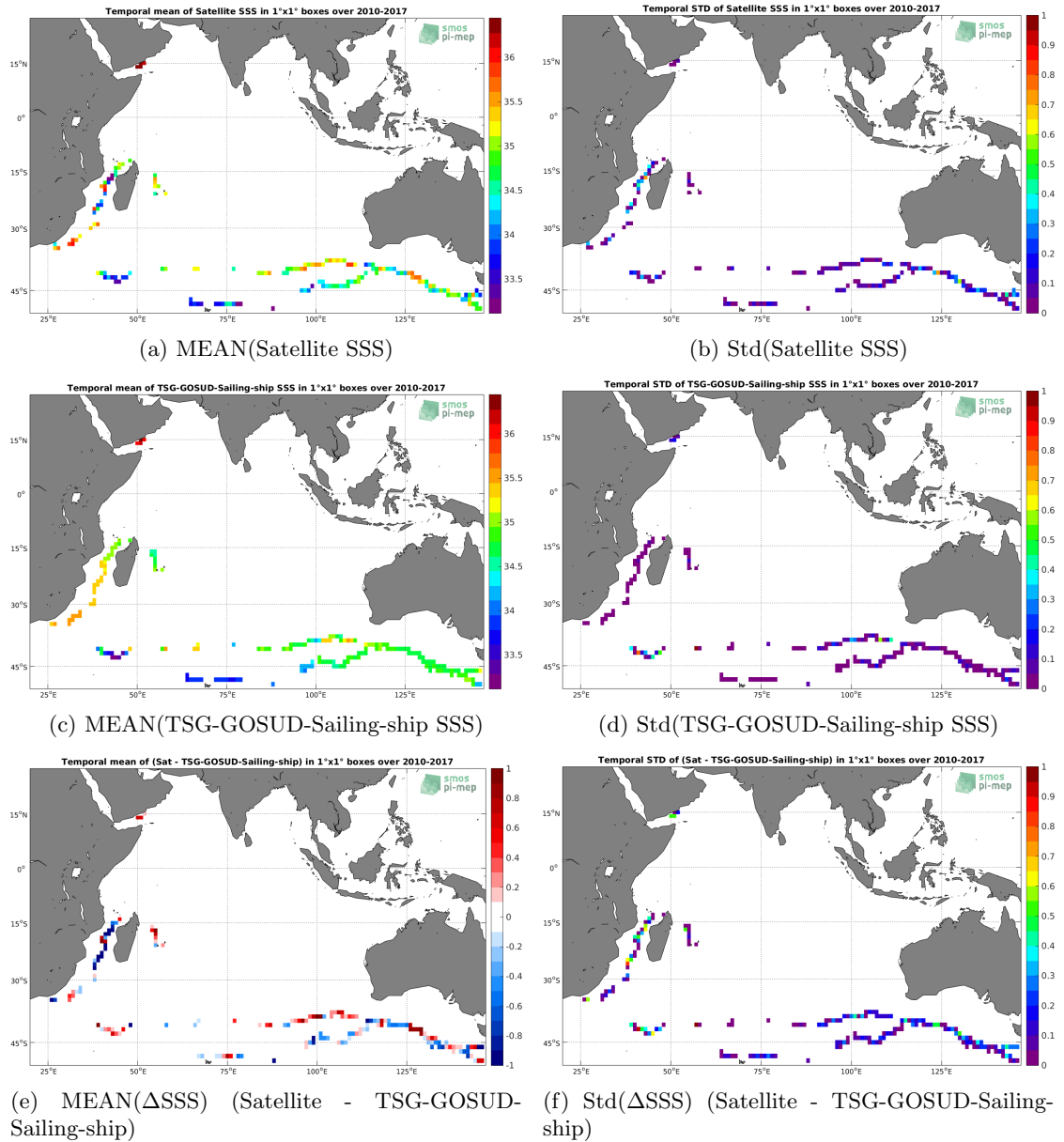
Figure 6: Temporal mean (left) and Std (right) of SSS from SMOS L3 v2 - Daily - 0.5 Deg (CATDS-CECOS-IFREMER) (top), TSG-GOSUD-Sailing-ship (middle), and of \Delta SSS (Satellite - TSG-GOSUD-Sailing-ship). Only match-up pairs are used to generate these maps.
