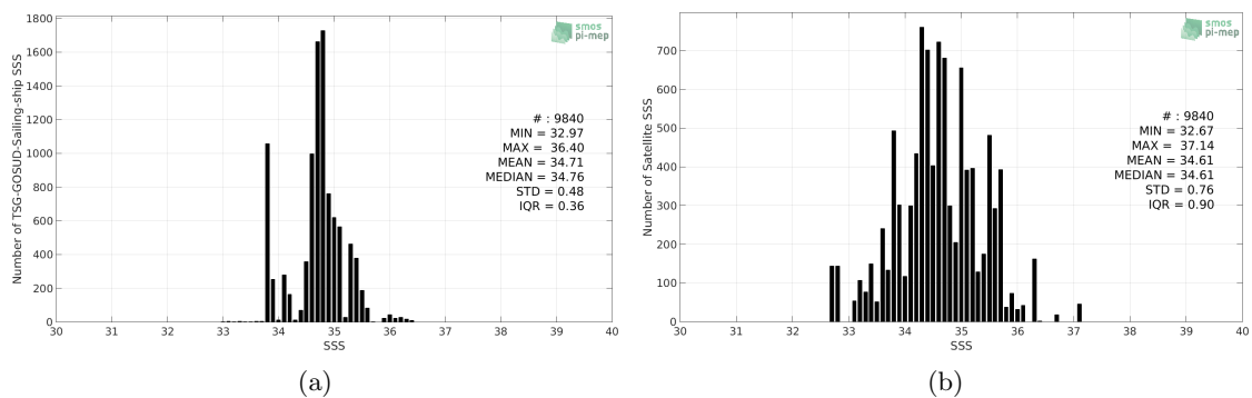
Figure 2: Histograms of SSS from TSG-GOSUD-Sailing-ship (a) and SMOS-L3-CATDS-CECOS-IFREMER-V2-1DAY-0.5DEG (b) considering all match-up pairs per bins of 0.1 over the Indian Ocean Pi-MEP region and for the full satellite product period.
