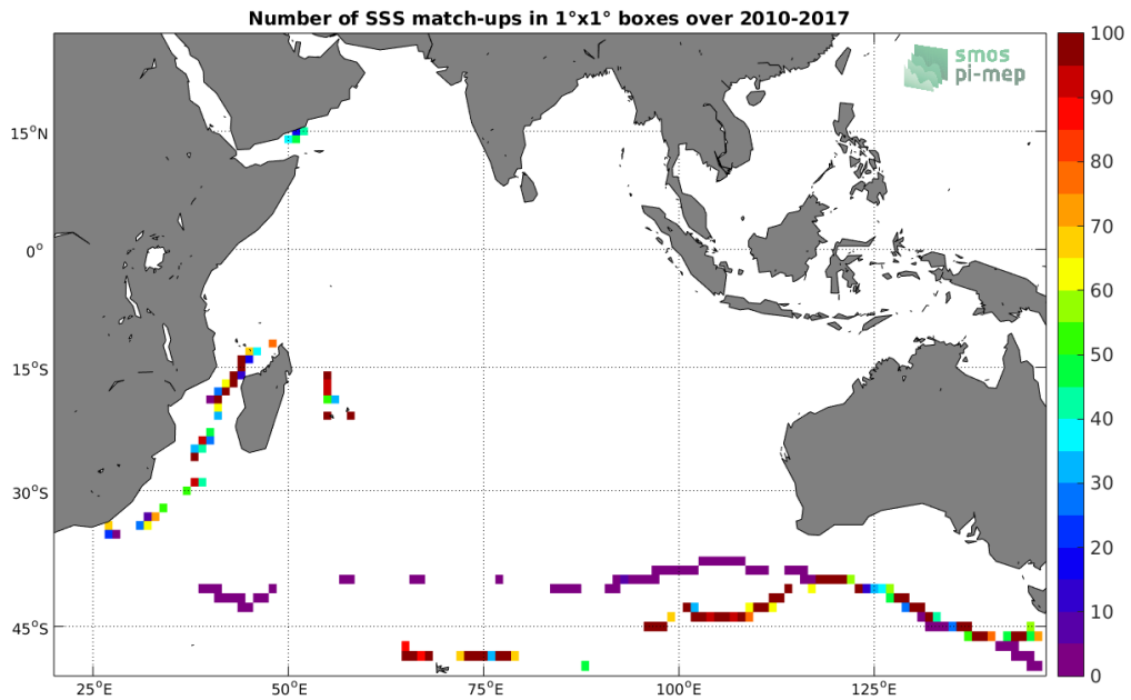
Figure 4: Number of SSS match-ups between TSG-GOSUD-Sailing-ship SSS and the SMOS-L3-CATDS-CECOS-IFREMER-V2-1DAY-0.5DEG SSS product for the Indian Ocean Pi-MEP region over 1^\circ \times 1^\circ boxes and for the full satellite product period.
