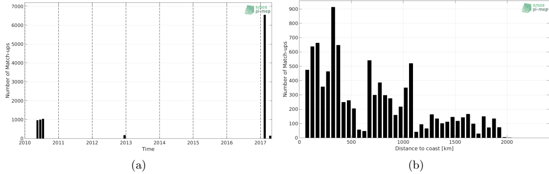
Figure 1: Number of match-ups between TSG-GOSUD-Sailing-ship and SMOS-L3-CATDS-CECOS-IFREMER-V2-1DAY-0.5DEG SSS as a function of time (a) and as function of the distance to coast (b) over the Indian Ocean Pi-MEP region and for the full satellite product period.
