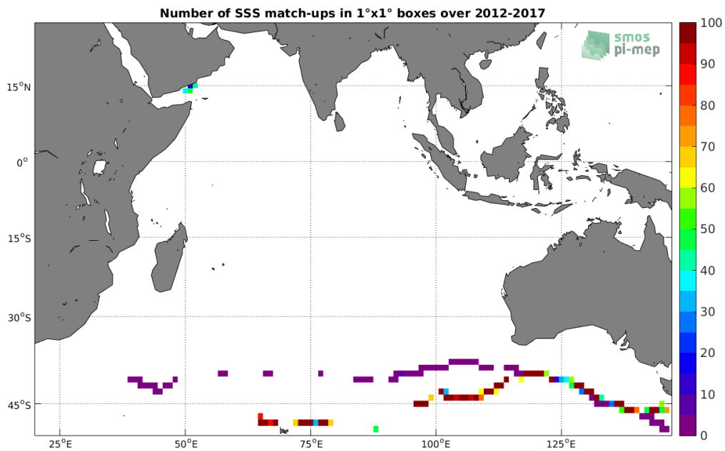
Figure 4: Number of SSS match-ups between TSG-GOSUD-Sailing-ship SSS and the SMOS-L3-CATDS-CECOS-IFREMER-V2-1DAY-0.5DEG SSS product for the Indian Ocean Pi-MEP region over 1^{\circ} \times 1^{\circ} boxes and for the full satellite product period.
