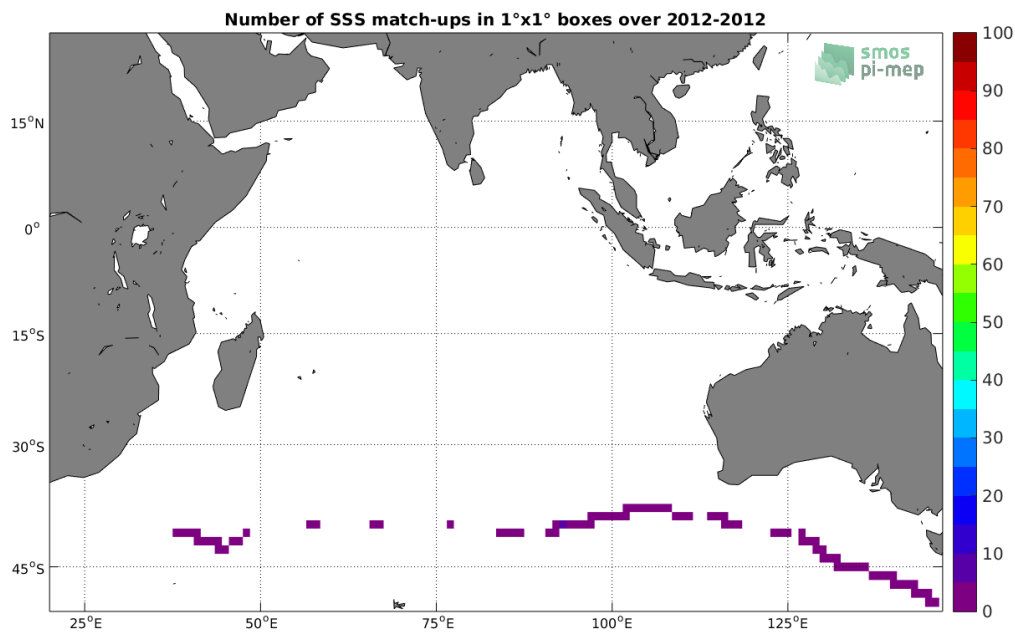
Figure 4: Number of SSS match-ups between TSG-GOSUD-Sailing-ship SSS and the SMOS-L3-CATDS-CECOS-IFREMER-V2-1DAY-0.5DEG SSS product for the Indian Ocean Pi-MEP region over 1^\circ \times 1^\circ boxes and for the full satellite product period.
