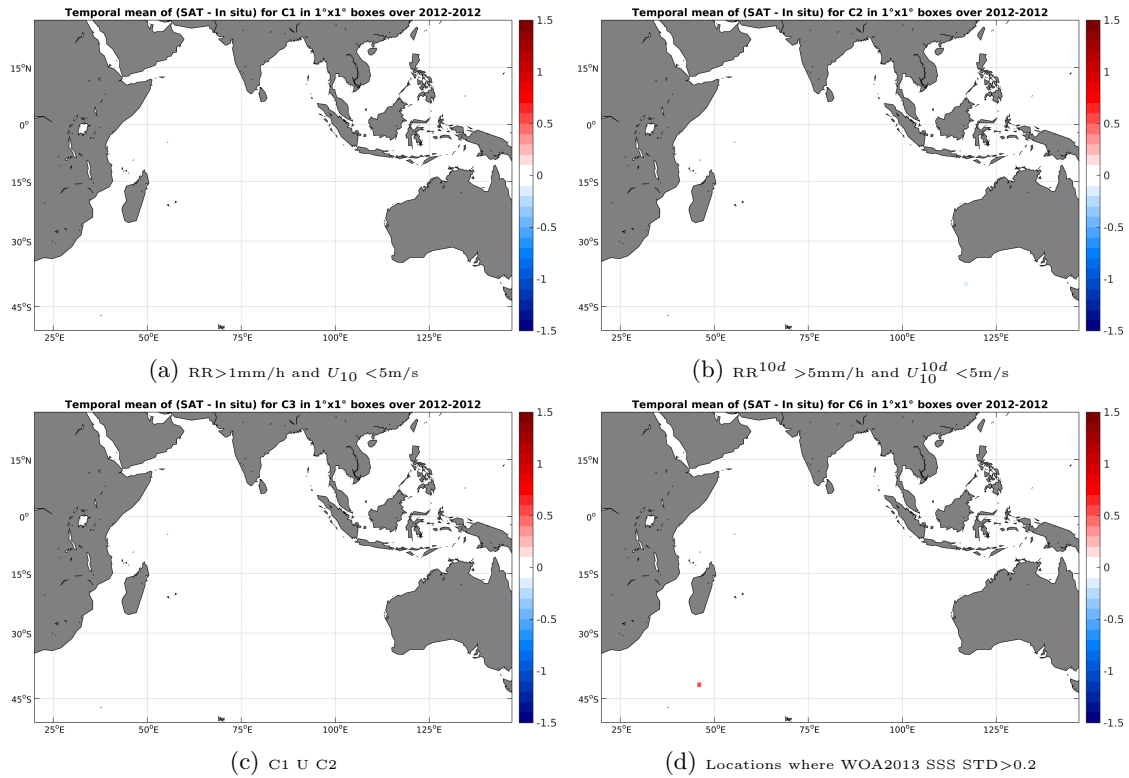
Figure 12: Temporal mean gridded over spatial boxes of size 1°x1° of \Delta SSS (SMOS-L3-CATDS-CECOS-IFREMER-V2-1DAY-0.5DEG - TSG-GOSUD-Sailing-ship) for 4 different subdatasets corresponding to: RR > 1mm/h and U_{10} < 5\text{m/s} (a), RR^{10d} > 5\text{mm/h} and U_{10}^{10d} < 5\text{m/s} (b), C1 U C2 (c), Locations where WOA2013 SSS STD > 0.2 (d).
