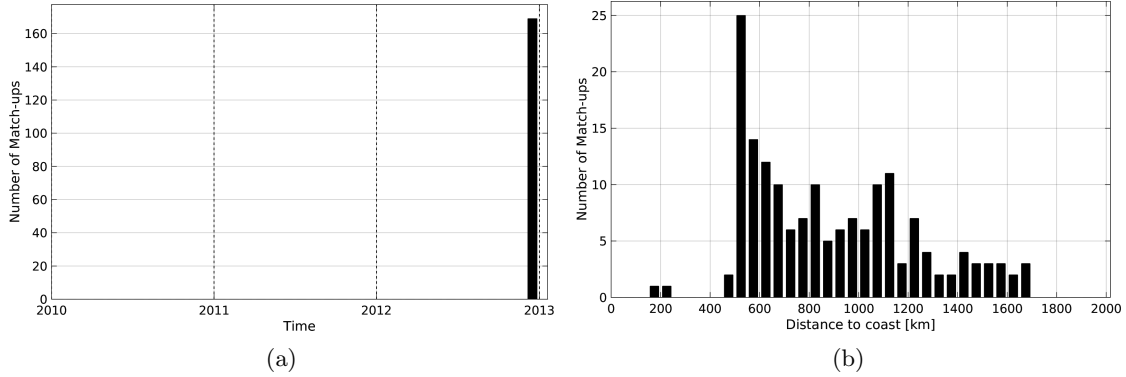
Figure 1: Number of match-ups between TSG-GOSUD-Sailing-ship and SMOS-L3-CATDS-CECOS-IFREMER-V2-1DAY-0.5DEG SSS as a function of time (a) and as function of the distance to coast (b) over the Indian Ocean Pi-MEP region and for the full satellite product period.
