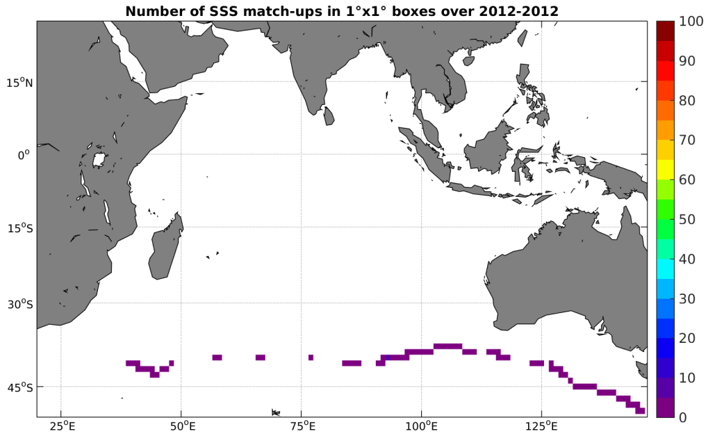
Figure 4: Number of SSS match-ups between TSG-GOSUD-Sailing-ship SSS and the SMOS-L3-CATDS-CECOS-IFREMER-V2-1DAY-0.5deg SSS product for the Indian Ocean Pi-MEP region over 1°x1° boxes and for the full satellite product period.
