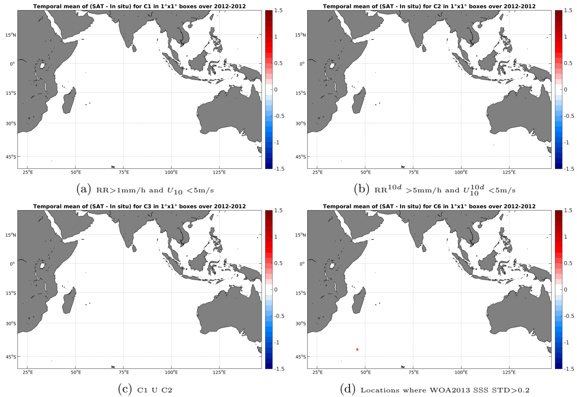
Figure 12: Temporal mean gridded over spatial boxes of size 1°x1° of \Delta SSS (SMOS-L3-CATDS-CECOS-IFREMER-V2-1DAY-0.5deg - TSG-GOSUD-Sailing-ship) for 4 different subdatasets corresponding to:RR>1mm/h and U_{10} < 5m/s (a), RR^{10d} > 5mm/h and U_{10}^{10d} < 5m/s (b), C1 U C2 (c),Locations where WOA2013 SSS STD>0.2 (d).
