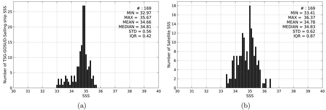
Figure 2: Histograms of SSS from TSG-GOSUD-Sailing-ship (a) and SMOS-L3-CATDS-CECOS-IFREMER-V2-1DAY-0.5deg (b) considering all match-up pairs per bins of 0.1 over the Indian Ocean Pi-MEP region and for the full satellite product period.
