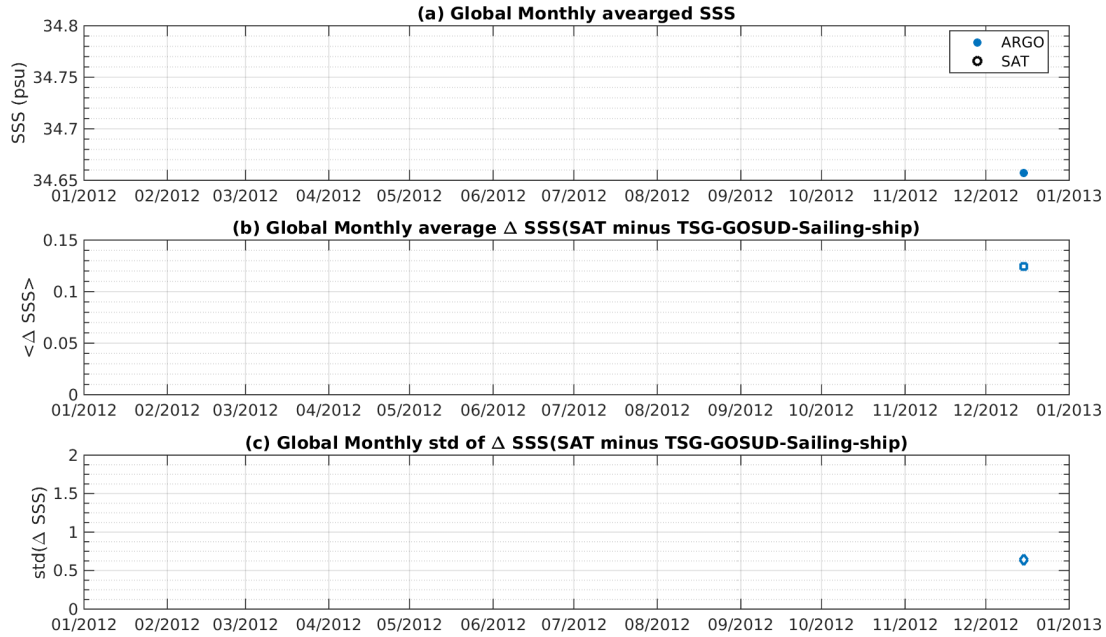
Figure 7: Time series of the monthly averaged mean SSS (top), mean \Delta SSS (Satellite - TSG-GOSUD-Sailing-ship) and STD of \Delta SSS (Satellite - TSG-GOSUD-Sailing-ship) over the Indian Ocean Pi-MEP region considering all match-ups collected by the Pi-MEP platform.
