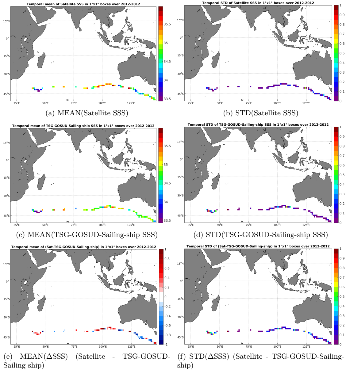
Figure 6: Temporal mean (left) and STD (right) of SSS from SMOS-L3-CATDS-CECOS-IFREMER-V2-1DAY-0.5deg (top), TSG-GOSUD-Sailing-ship (middle), and of \Delta SSS (Satellite - TSG-GOSUD-Sailing-ship). Only match-up pairs are used to generate these maps.
