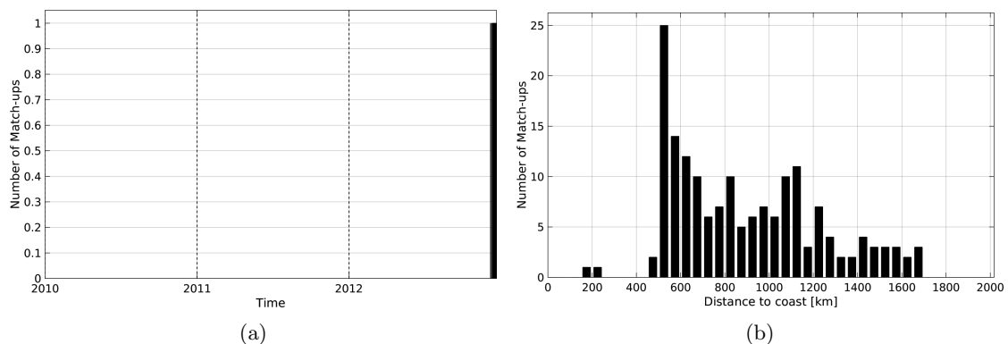
Figure 1: Number of match-ups between TSG-GOSUD-Sailing-ship and SMOS-L3-CATDS-CECOS-IFREMER-V2-1DAY-0.5deg SSS as a function of time (a) and as function of the distance to coast (b) over the Indian Ocean Pi-MEP region and for the full satellite product period.
