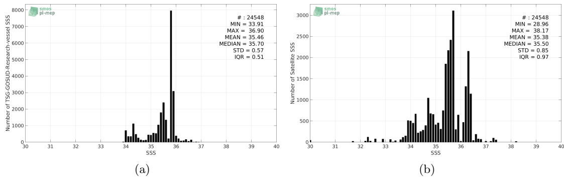
Figure 2: Histograms of SSS from TSG-GOSUD-Research-vessel (a) and SMOS-L3-CATDS-CECOS-IFREMER-V2-1DAY-0.5DEG (b) considering all match-up pairs per bins of 0.1 over the Indian Ocean Pi-MEP region and for the full satellite product period.
