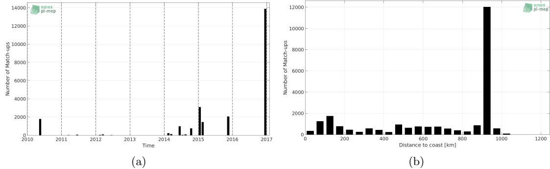
Figure 1: Number of match-ups between TSG-GOSUD-Research-vessel and SMOS-L3-CATDS-CECOS-IFREMER-V2-1DAY-0.5DEG SSS as a function of time (a) and as function of the distance to coast (b) over the Indian Ocean Pi-MEP region and for the full satellite product period.
