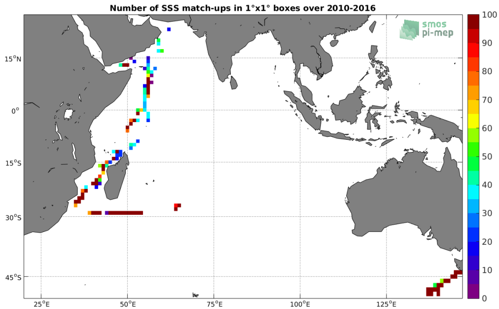
Figure 4: Number of SSS match-ups between TSG-GOSUD-Research-vessel SSS and the SMOS-L3-CATDS-CECOS-IFREMER-V2-1DAY-0.5DEG SSS product for the Indian Ocean Pi-MEP region over 1^\circ \times 1^\circ boxes and for the full satellite product period.
