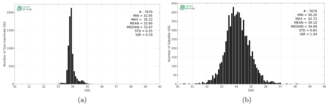
Figure 2: Histograms of SSS from Sea mammals (a) and SMOS-L3-CATDS-CECOS-IFREMER-V2-1DAY-0.5DEG (b) considering all match-up pairs per bins of 0.1 over the Indian Ocean Pi-MEP region and for the full satellite product period.
