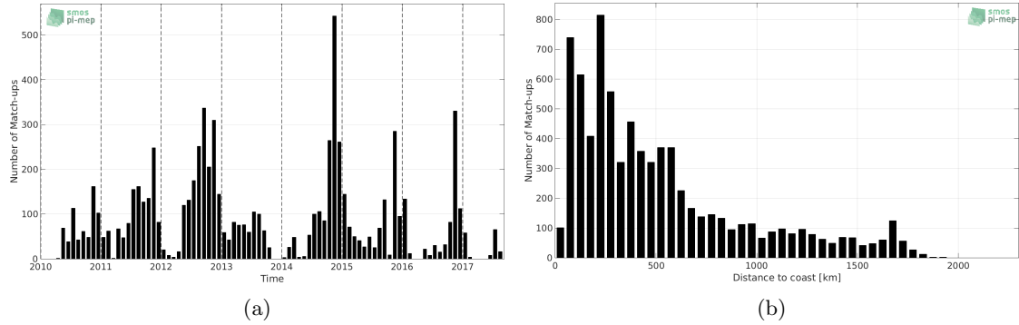
Figure 1: Number of match-ups between Sea mammals and SMOS-L3-CATDS-CECOS-IFREMER-V2-1DAY-0.5DEG SSS as a function of time (a) and as function of the distance to coast (b) over the Indian Ocean Pi-MEP region and for the full satellite product period.
