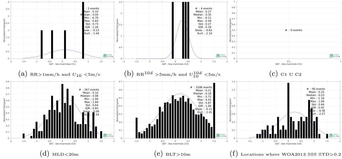
Figure 13: Normalized histogram of \Delta SSS (SMOS-L3-CATDS-CECOS-IFREMER-V2-1DAY-0.5DEG - Sea mammals) for 6 different subdatasets corresponding to: RR > 1\text{mm/h} and U_{10} < 5\text{m/s} (a), RR^{10d} > 5\text{mm/h} and U_{10}^{10d} < 5\text{m/s} (b), C1 \cup C2 (c), MLD < 20\text{m} (d), BLT > 10\text{m} (e), Locations where WOA2013 SSS STD > 0.2 (f).
