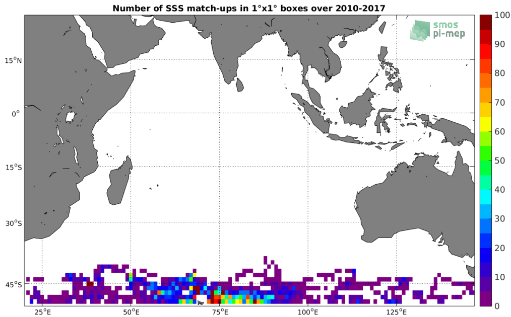
Figure 4: Number of SSS match-ups between Sea mammals SSS and the SMOS-L3-CATDS-CECOS-IFREMER-V2-1DAY-0.5DEG SSS product for the Indian Ocean Pi-MEP region over 1^\circ \times 1^\circ boxes and for the full satellite product period.
