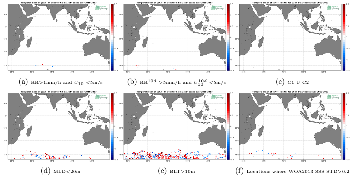
Figure 12: Temporal mean gridded over spatial boxes of size 1^\circ \times 1^\circ of \Delta\text{SSS} (SMOS-L3-CATDS-CECOS-IFREMER-V2-1DAY-0.5DEG - Sea mammals) for 6 different subdatasets corresponding to: RR > 1\text{mm/h} and U_{10} < 5\text{m/s} (a), RR^{10d} > 5\text{mm/h} and U_{10}^{10d} < 5\text{m/s} (b), C1 U C2 (c), MLD < 20\text{m} (d), BLT > 10\text{m} (e), Locations where WOA2013 SSS STD > 0.2 (f).
