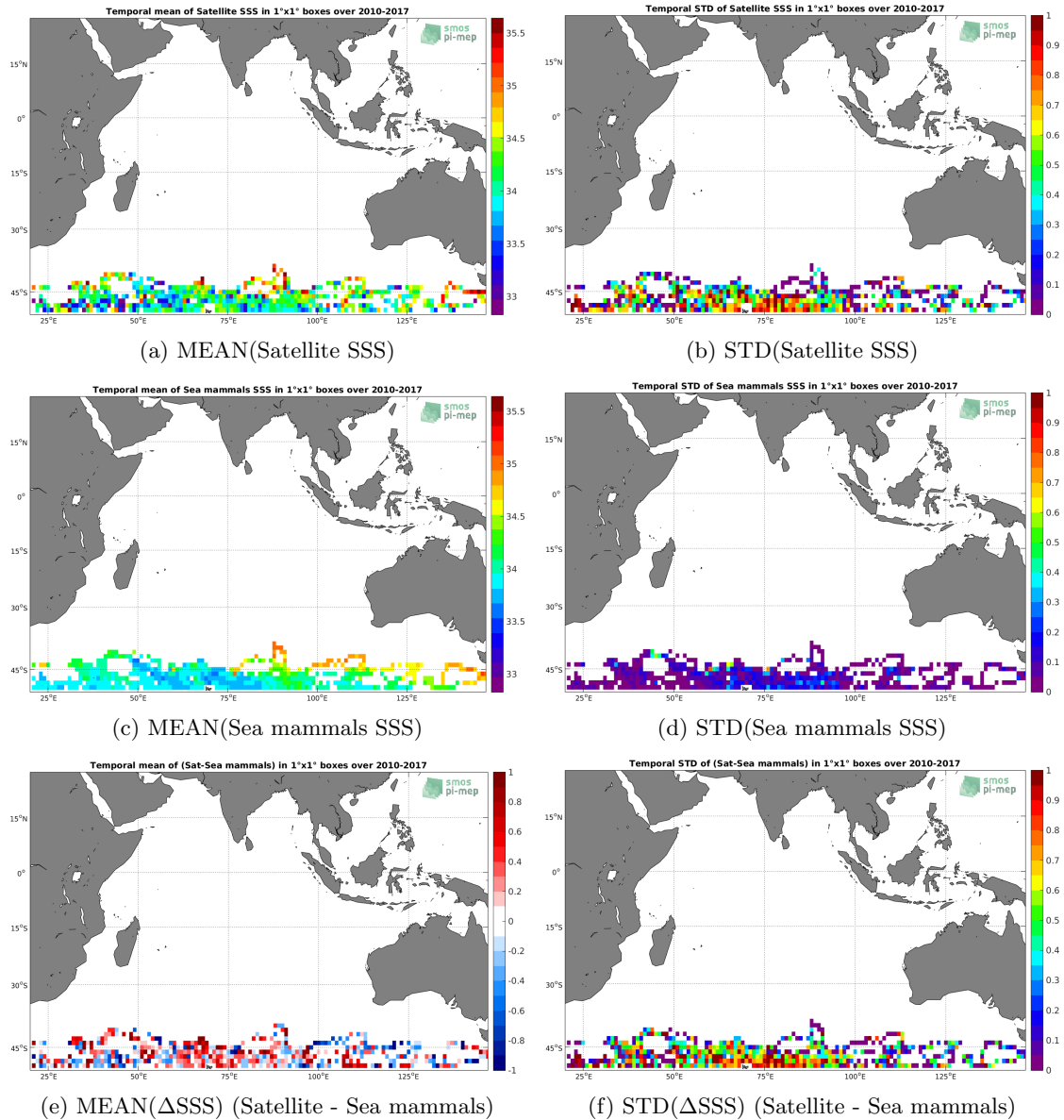
Figure 6: Temporal mean (left) and STD (right) of SSS from SMOS-L3-CATDS-CECOS-IFREMER-V2-1DAY-0.5DEG (top), Sea mammals (middle), and of \Delta SSS (Satellite - Sea mammals). Only match-up pairs are used to generate these maps.
