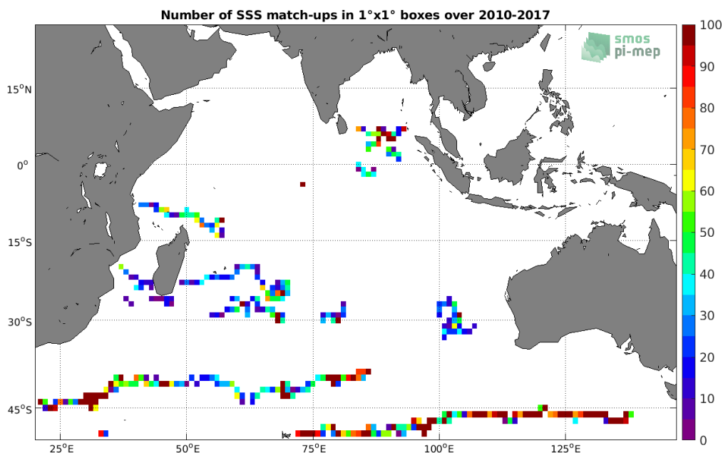
Figure 3: Number of SSS match-ups between Surface drifters SSS and the SMOS SSS L3 v2 - Daily - 0.5 Deg (CATDS-CECOS-IFREMER) SSS product for the Indian Ocean Pi-MEP region over 1^\circ \times 1^\circ boxes and for the full satellite product period.
