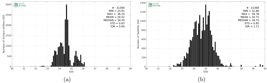
Figure 2: Histograms of SSS from Surface drifters (a) and SMOS-L3-CATDS-CECOS-IFREMER-V2-1DAY-0.5DEG (b) considering all match-up pairs per bins of 0.1 over the Indian Ocean Pi-MEP region and for the full satellite product period.
