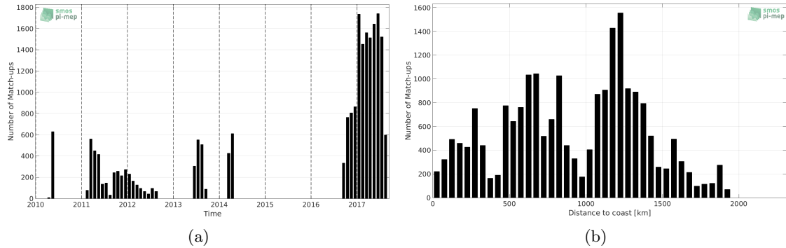
Figure 1: Number of match-ups between Surface drifters and SMOS-L3-CATDS-CECOS-IFREMER-V2-1DAY-0.5DEG SSS as a function of time (a) and as function of the distance to coast (b) over the Indian Ocean Pi-MEP region and for the full satellite product period.
