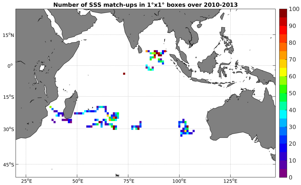
Figure 3: Number of SSS match-ups between Surface drifters SSS and the SMOS-L3-CATDS-CECOS-IFREMER-V2-1DAY-0.5DEG SSS product for the Indian Ocean Pi-MEP region over 1°x1° boxes and for the full satellite product period.
