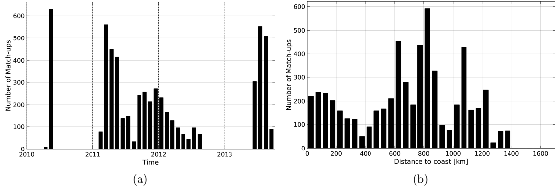
Figure 1: Number of match-ups between Surface drifters and SMOS-L3-CATDS-CECOS-IFREMER-V2-1DAY-0.5DEG SSS as a function of time (a) and as function of the distance to coast (b) over the Indian Ocean Pi-MEP region and for the full satellite product period.
