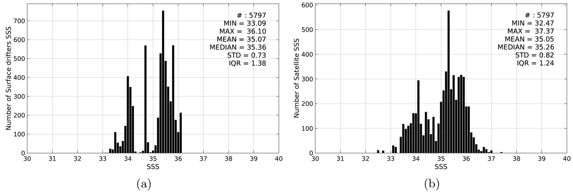
Figure 2: Histograms of SSS from Surface drifters (a) and SMOS-L3-CATDS-CECOS-IFREMER-V2-1DAY-0.5deg (b) considering all match-up pairs per bins of 0.1 over the Indian Ocean Pi-MEP region and for the full satellite product period.
