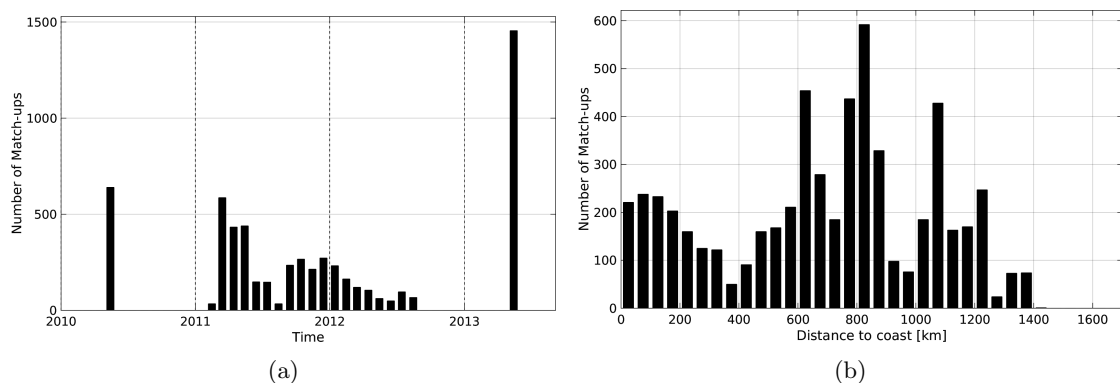
Figure 1: Number of match-ups between Surface drifters and SMOS-L3-CATDS-CECOS-IFREMER-V2-1DAY-0.5deg SSS as a function of time (a) and as function of the distance to coast (b) over the Indian Ocean Pi-MEP region and for the full satellite product period.
