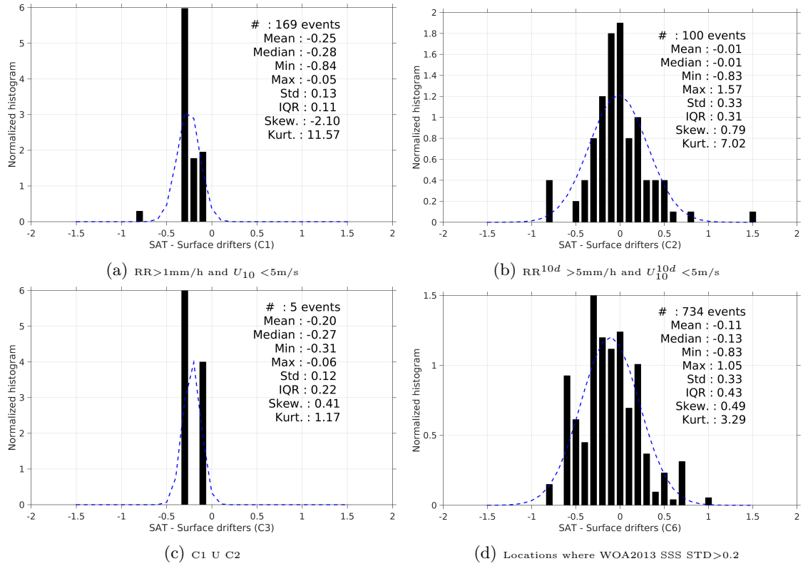
Figure 12: Normalized histogram of \Delta SSS (SMOS-L3-CATDS-CECOS-IFREMER-V2-1DAY-0.5deg - Surface drifters) for 6 different subdatasets corresponding to: RR > 1mm/h and U_{10} < 5\text{m/s} (a), RR^{10d} > 5\text{mm/h} and U_{10}^{10d} < 5\text{m/s} (b), C1 U C2 (c), Locations where WOA2013 SSS STD > 0.2 (d).
