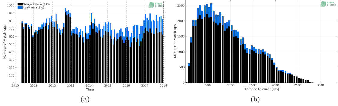
Figure 1: Number of match-ups between Argo and SMOS SSS L3 v2 - Daily - 0.5 Deg (CATDS-CECOS-IFREMER) SSS as a function of time (a) and as function of the distance to coast (b) over the Indian Ocean Pi-MEP region and for the full satellite product period.
