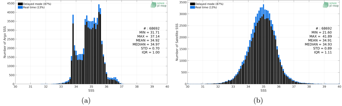
Figure 2: Histograms of SSS from Argo (a) and SMOS SSS L3 v2 - Daily - 0.5 Deg (CATDS-CECOS-IFREMER) (b) considering all match-up pairs per bins of 0.1 over the Indian Ocean Pi-MEP region and for the full satellite product period.
