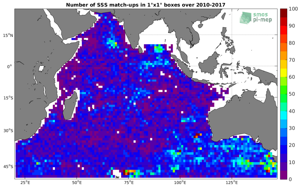
Figure 4: Number of SSS match-ups between Argo SSS and the SMOS SSS L3 v2 - Daily - 0.5 Deg (CATDS-CECOS-IFREMER) SSS product for the Indian Ocean Pi-MEP region over 1°x1° boxes and for the full satellite product period.
