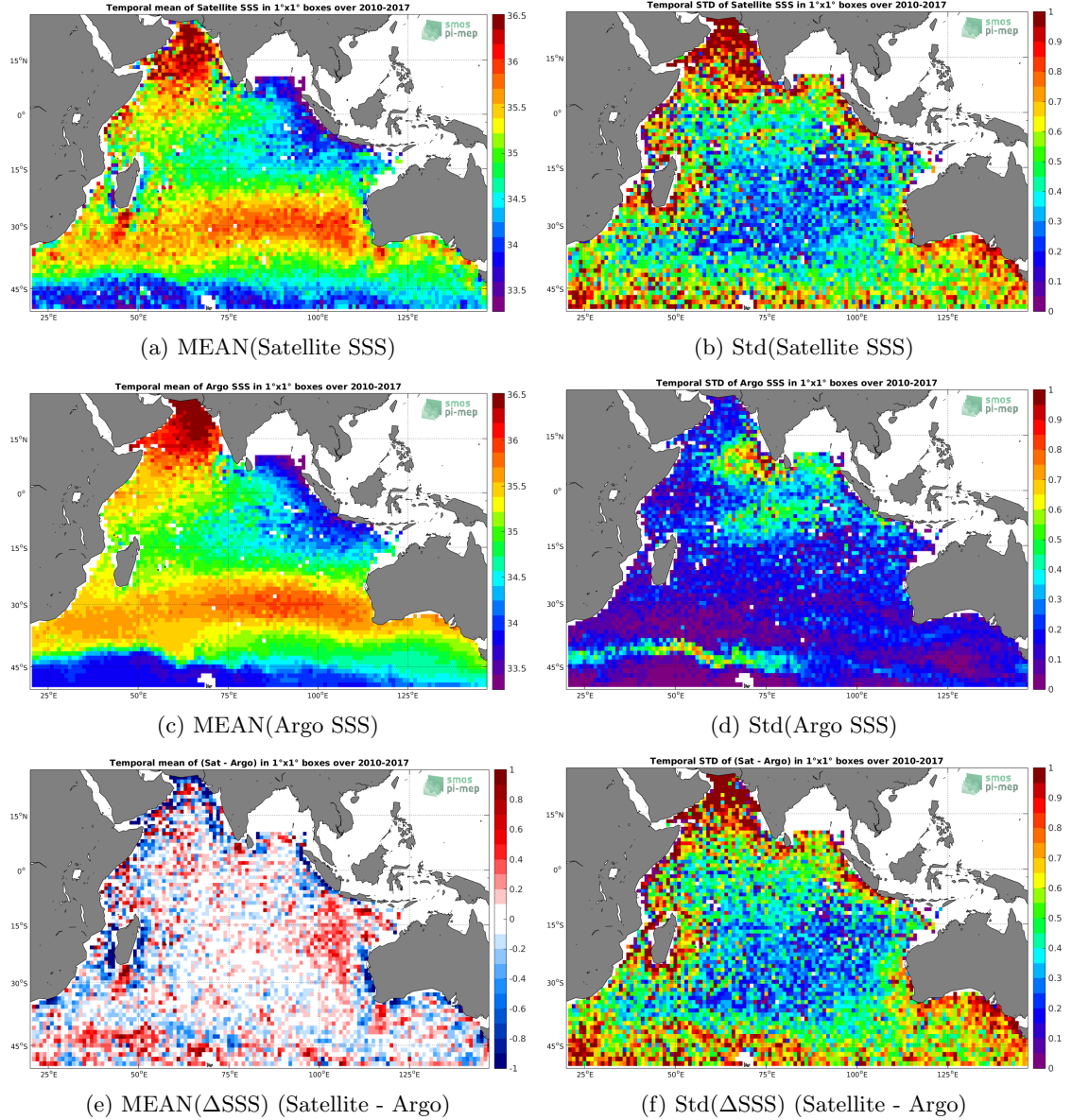
Figure 6: Temporal mean (left) and Std (right) of SSS from SMOS L3 v2 - Daily - 0.5 Deg (CATDS-CECOS-IFREMER) (top), Argo (middle), and of \Delta SSS (Satellite - Argo). Only match-up pairs are used to generate these maps.
