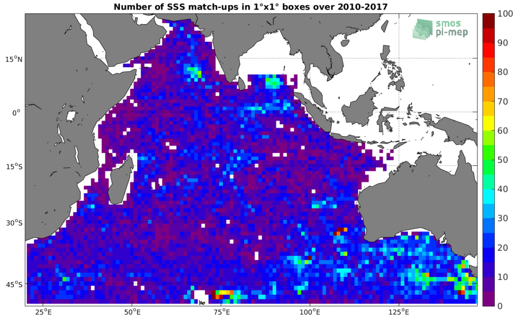
Figure 4: Number of SSS match-ups between Argo SSS and the SMOS L3 v2 - Daily - 0.5 Deg (CATDS-CECOS-IFREMER) SSS product for the Indian Ocean Pi-MEP region over 1°x1° boxes and for the full satellite product period.
