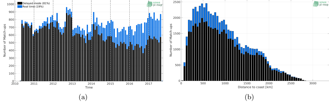
Figure 1: Number of match-ups between Argo and SMOS L3 v2 - Daily - 0.5 Deg (CATDS-CECOS-IFREMER) SSS as a function of time (a) and as function of the distance to coast (b) over the Indian Ocean Pi-MEP region and for the full satellite product period.
