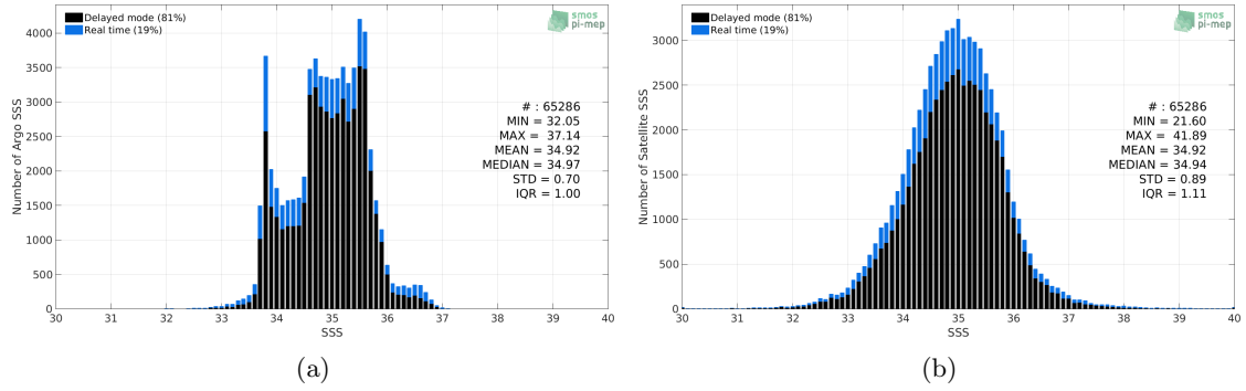
Figure 2: Histograms of SSS from Argo (a) and SMOS L3 v2 - Daily - 0.5 Deg (CATDS-CECOS-IFREMER) (b) considering all match-up pairs per bins of 0.1 over the Indian Ocean Pi-MEP region and for the full satellite product period.
