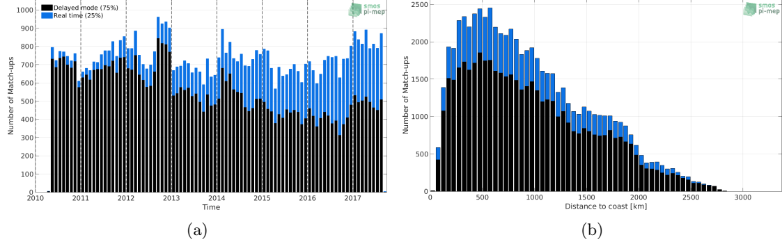
Figure 1: Number of match-ups between Argo and SMOS-L3-CATDS-CECOS-IFREMER-V2-1DAY-0.5DEG SSS as a function of time (a) and as function of the distance to coast (b) over the Indian Ocean Pi-MEP region and for the full satellite product period.
