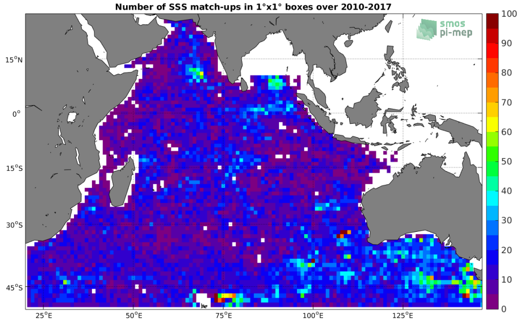
Figure 4: Number of SSS match-ups between Argo SSS and the SMOS-L3-CATDS-CECOS-IFREMER-V2-1DAY-0.5DEG SSS product for the Indian Ocean Pi-MEP region over 1°x1° boxes and for the full satellite product period.
