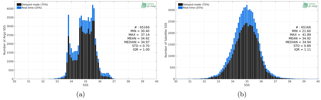
Figure 2: Histograms of SSS from Argo (a) and SMOS-L3-CATDS-CECOS-IFREMER-V2-1DAY-0.5DEG (b) considering all match-up pairs per bins of 0.1 over the Indian Ocean Pi-MEP region and for the full satellite product period.
