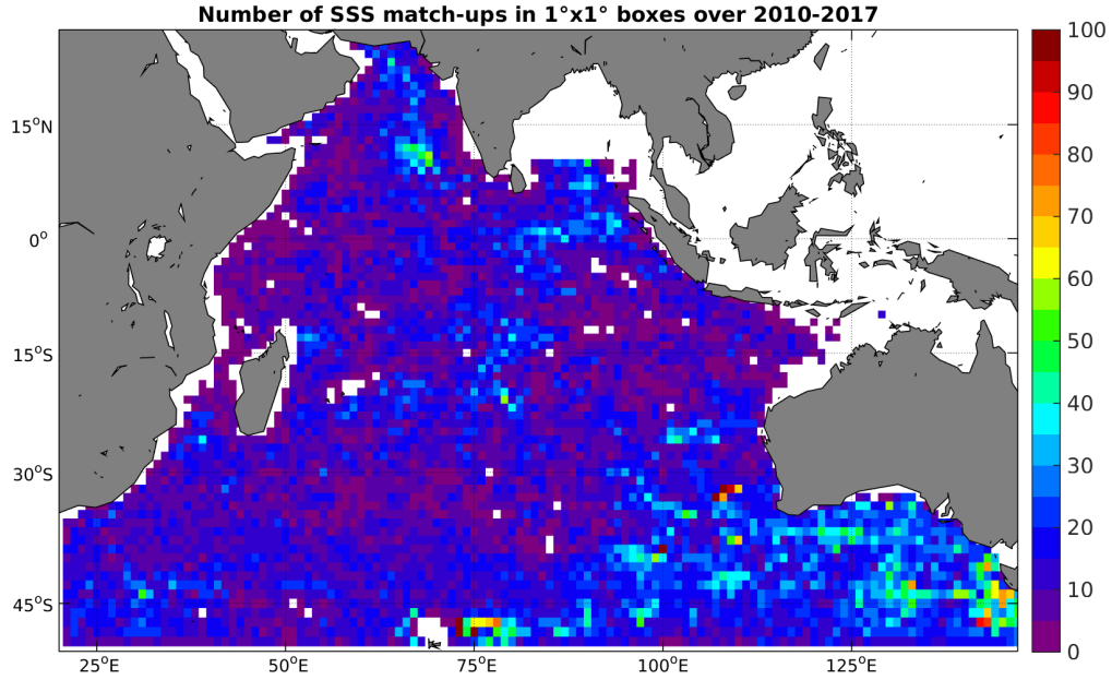
Figure 4: Number of SSS match-ups between Argo SSS and the SMOS-L3-CATDS-CECOS-IFREMER-V2-1DAY-0.5deg SSS product for the Indian Ocean Pi-MEP region over 1^\circ \times 1^\circ boxes and for the full satellite product period.
