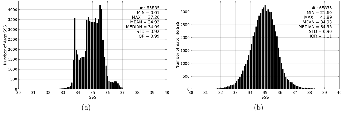
Figure 2: Histograms of SSS from Argo (a) and SMOS-L3-CATDS-CECOS-IFREMER-V2-1DAY-0.5deg (b) considering all match-up pairs per bins of 0.1 over the Indian Ocean Pi-MEP region and for the full satellite product period.
