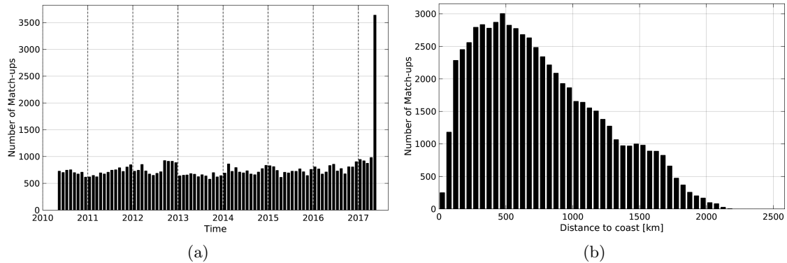
Figure 1: Number of match-ups between Argo and SMOS-L3-CATDS-CECOS-IFREMER-V2-1DAY-0.5deg SSS as a function of time (a) and as function of the distance to coast (b) over the Indian Ocean Pi-MEP region and for the full satellite product period.
