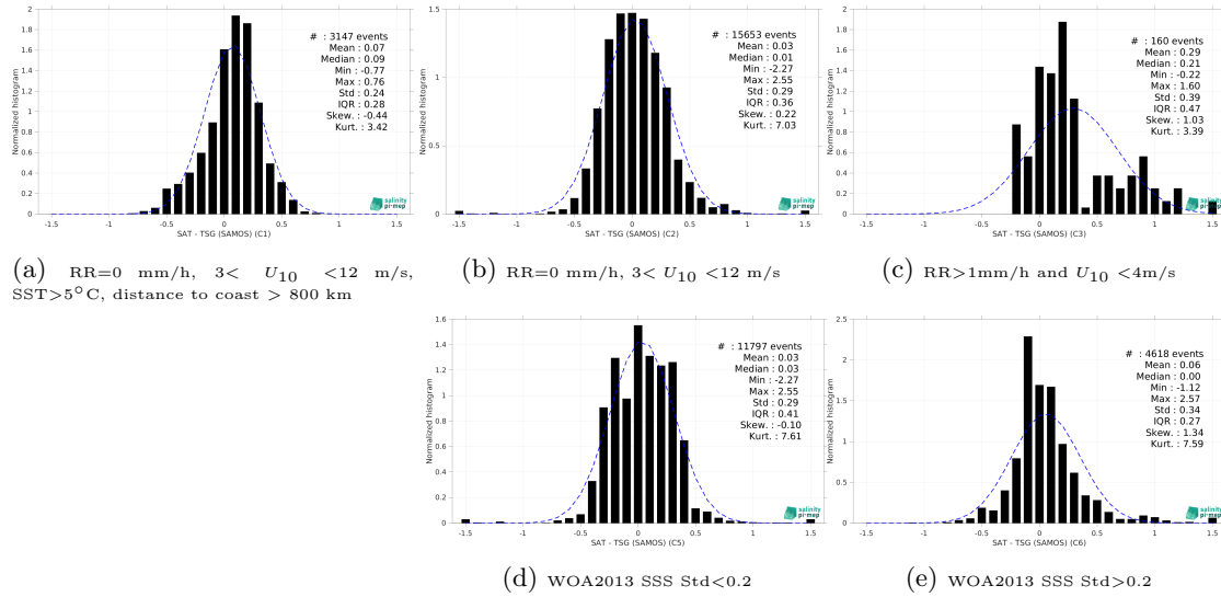
Figure 15: Normalized histogram of \Delta\text{SSS} (SMOS SSS L3 v335 - Monthly - 25 km (CATDS-CPDC) - TSG (SAMOS)) for 5 different subdatasets corresponding to: RR=0 mm/h, 3 < U_{10} < 12 m/s, SST>5°C, distance to coast > 800 km (a), RR=0 mm/h, 3 < U_{10} < 12 m/s (b), RR>1mm/h and U_{10} < 4 m/s (c), WOA2013 SSS Std<0.2 (d), WOA2013 SSS Std>0.2 (e).
