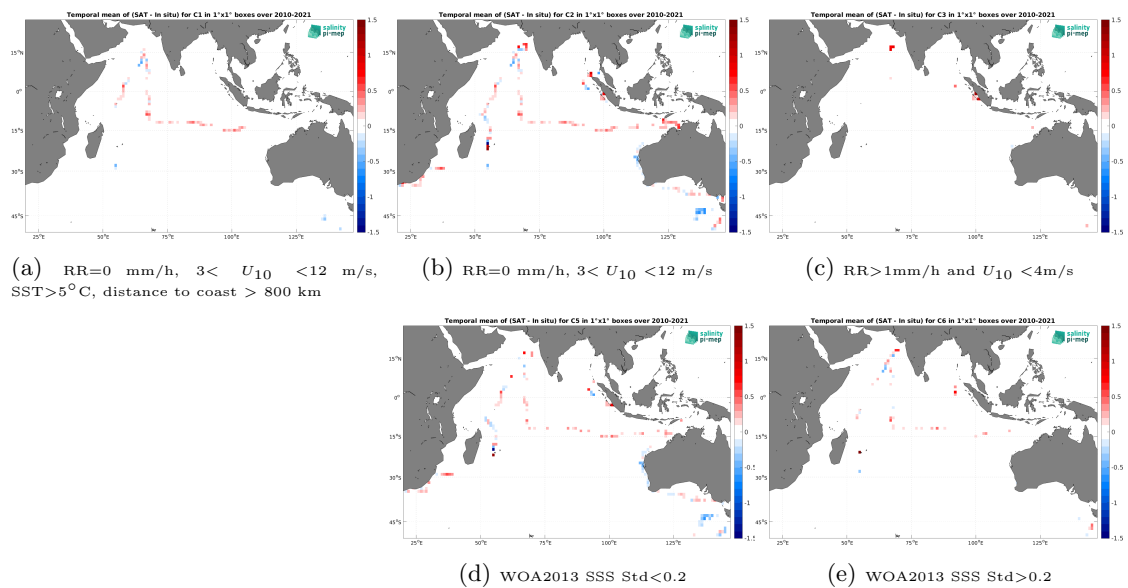
Figure 14: Temporal mean gridded over spatial boxes of size 1^\circ \times 1^\circ of \Delta SSS (SMOS SSS L3 v335 - Monthly - 25 km (CATDS-CPDC) - TSG (SAMOS)) for 5 different subdatasets corresponding to:RR=0 mm/h, 3 < U_{10} < 12 m/s, SST > 5^\circ\text{C} , distance to coast > 800 km (a), RR=0 mm/h, 3 < U_{10} < 12 m/s (b), RR > 1 mm/h and U_{10} < 4 m/s (c), WOA2013 SSS Std < 0.2 (d), WOA2013 SSS Std > 0.2 (e).
