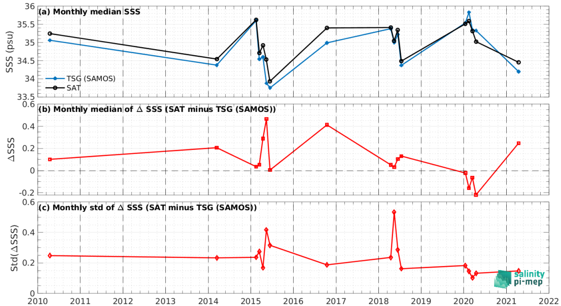
Figure 8: Time series of the monthly median SSS (top), median of \Delta SSS (Satellite - TSG (SAMOS)) and Std of \Delta SSS (Satellite - TSG (SAMOS)) over the Indian Ocean Pi-MEP region considering all match-ups collected by the Pi-MEP.
