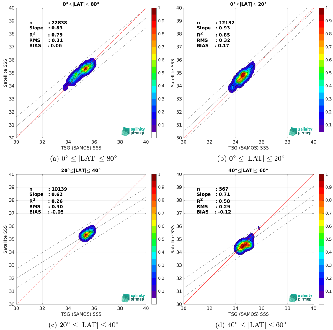
Figure 10: Contour maps of the concentration of SMOS SSS L3 v335 - Monthly - 25 km (CATDS-CPDC) SSS (y-axis) versus TSG (SAMOS) SSS (x-axis) at match-up pairs for different latitude bands. For each plot, the red line shows x=y . The black thin and dashed lines indicate a linear fit through the data cloud and the \pm 95\% confidence levels, respectively. The number match-up pairs n , the slope and R^2 coefficient of the linear fit, the root mean square (RMS) and the mean bias between satellite and in situ data are indicated for each latitude band in each plots.
