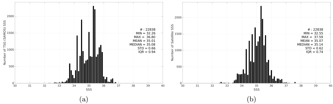
Figure 3: Histograms of SSS from TSG (SAMOS) (a) and SMOS SSS L3 v335 - Monthly - 25 km (CATDS-CPDC) (b) considering all match-up pairs per bins of 0.1 over the Indian Ocean Pi-MEP region and for the full satellite product period.
