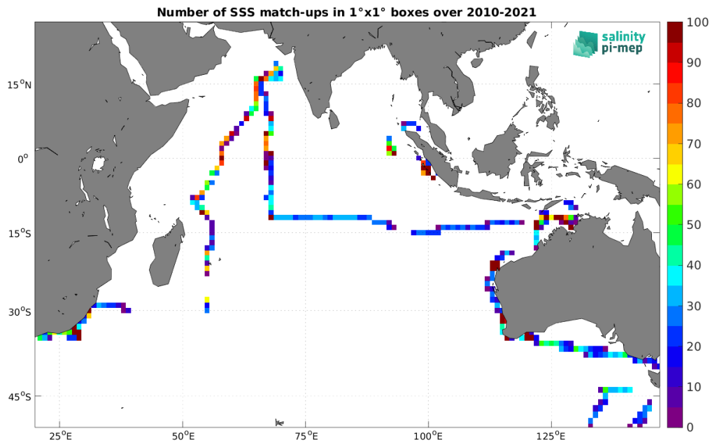
Figure 5: Number of SSS match-ups between TSG (SAMOS) SSS and the SMOS SSS L3 v335 - Monthly - 25 km (CATDS-CPDC) SSS product for the Indian Ocean Pi-MEP region over 1^\circ \times 1^\circ boxes and for the full satellite product period.
