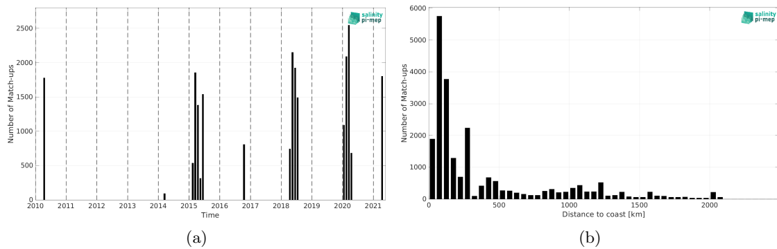
Figure 2: Number of match-ups between TSG (SAMOS) and SMOS SSS L3 v335 - Monthly - 25 km (CATDS-CPDC) SSS as a function of time (a) and as function of the distance to coast (b) over the Indian Ocean Pi-MEP region and for the full satellite product period.
