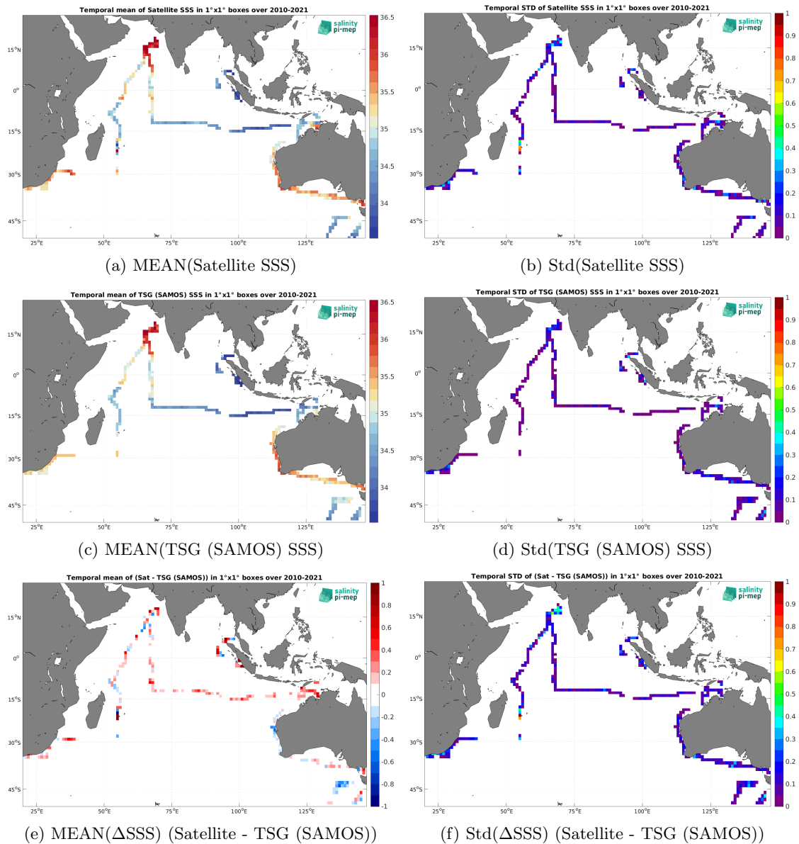
Figure 7: Temporal mean (left) and Std (right) of SSS from SMOS SSS L3 v335 - Monthly - 25 km (CATDS-CPDC) (top), TSG (SAMOS) (middle), and of \Delta SSS (Satellite - TSG (SAMOS)). Only match-up pairs are used to generate these maps.
