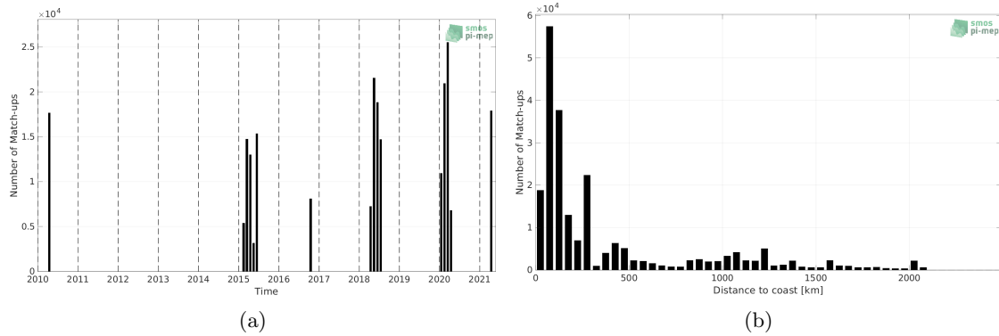
Figure 1: Number of match-ups between TSG (SAMOS) and SMOS SSS L3 v335 - Monthly - 25 km (CATDS-CPDC) SSS as a function of time (a) and as function of the distance to coast (b) over the Indian Ocean Pi-MEP region and for the full satellite product period.
