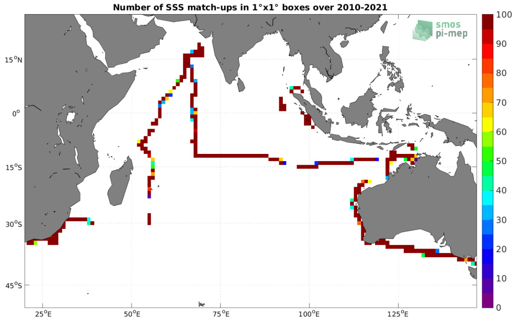
Figure 4: Number of SSS match-ups between TSG (SAMOS) SSS and the SMOS SSS L3 v335 - Monthly - 25 km (CATDS-CPDC) SSS product for the Indian Ocean Pi-MEP region over 1^\circ \times 1^\circ boxes and for the full satellite product period.
