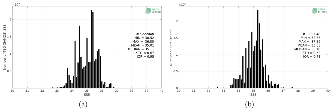
Figure 2: Histograms of SSS from TSG (SAMOS) (a) and SMOS SSS L3 v335 - Monthly - 25 km (CATDS-CPDC) (b) considering all match-up pairs per bins of 0.1 over the Indian Ocean Pi-MEP region and for the full satellite product period.
