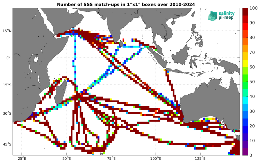
Figure 5: Number of SSS match-ups between TSG (LEGOS-DM) SSS and the SMOS SSS L3 v335 - Monthly - 25 km (CATDS-CPDC) SSS product for the Indian Ocean Pi-MEP region over 1^\circ \times 1^\circ boxes and for the full satellite product period.
