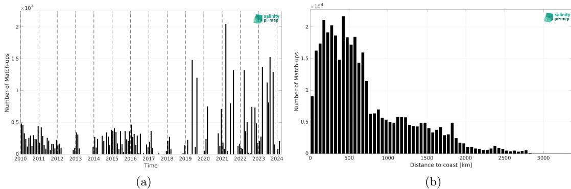
Figure 2: Number of match-ups between TSG (LEGOS-DM) and SMOS SSS L3 v335 - Monthly - 25 km (CATDS-CPDC) SSS as a function of time (a) and as function of the distance to coast (b) over the Indian Ocean Pi-MEP region and for the full satellite product period.
