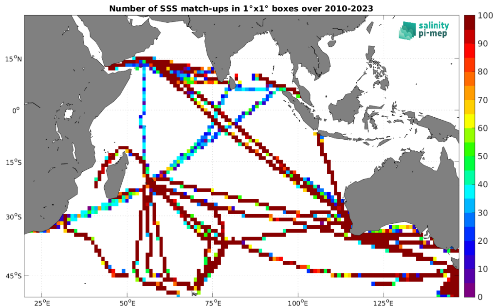
Figure 5: Number of SSS match-ups between TSG (LEGOS-DM) SSS and the SMOS SSS L3 v335 - Monthly - 25 km (CATDS-CPDC) SSS product for the Indian Ocean Pi-MEP region over 1^\circ \times 1^\circ boxes and for the full satellite product period.
