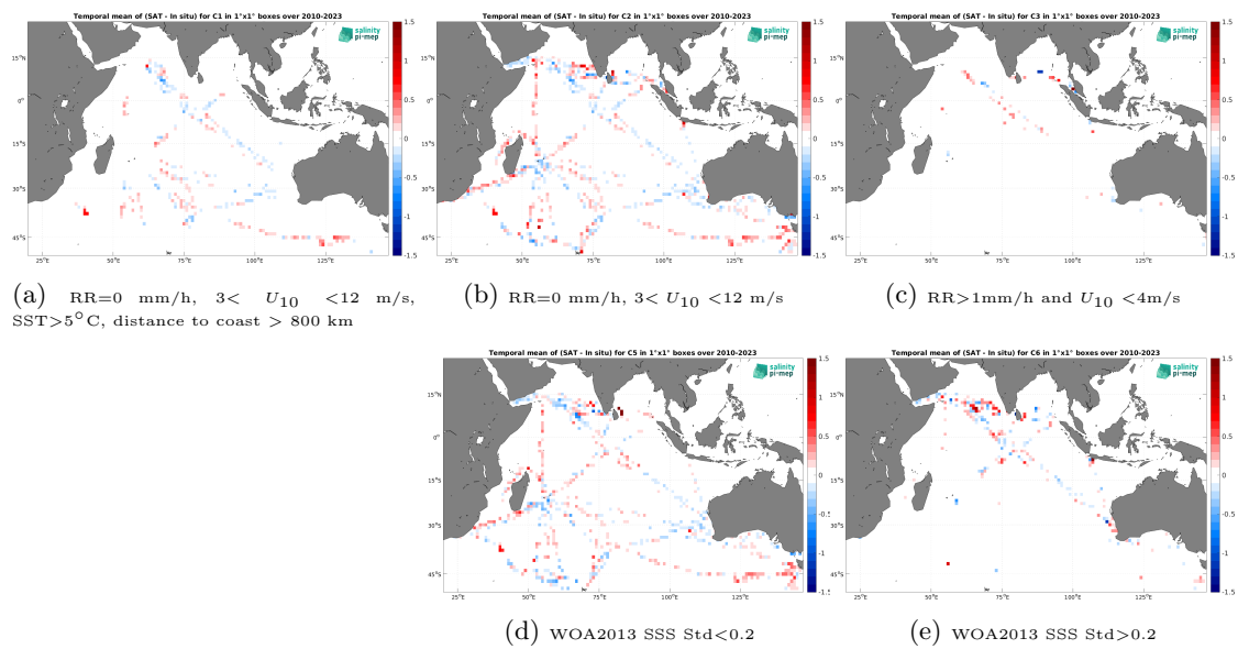
Figure 14: Temporal mean gridded over spatial boxes of size 1^\circ \times 1^\circ of \Delta SSS (SMOS SSS L3 v335 - Monthly - 25 km (CATDS-CPDC) - TSG (LEGOS-DM)) for 5 different subdatasets corresponding to:RR=0 mm/h, 3 < U_{10} < 12 m/s, SST >5^\circ\text{C} , distance to coast > 800 km (a), RR=0 mm/h, 3 < U_{10} < 12 m/s (b), RR >1 mm/h and U_{10} < 4 m/s (c), WOA2013 SSS Std <0.2 (d), WOA2013 SSS Std >0.2 (e).
