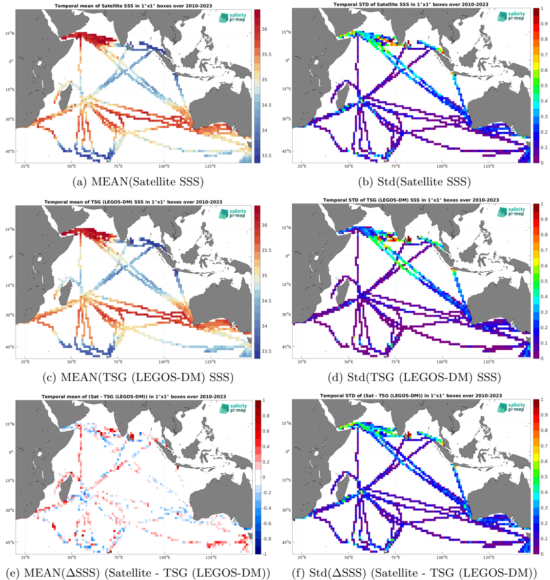
Figure 7: Temporal mean (left) and Std (right) of SSS from SMOS SSS L3 v335 - Monthly - 25 km (CATDS-CPDC) (top), TSG (LEGOS-DM) (middle), and of \Delta SSS (Satellite - TSG (LEGOS-DM)). Only match-up pairs are used to generate these maps.
