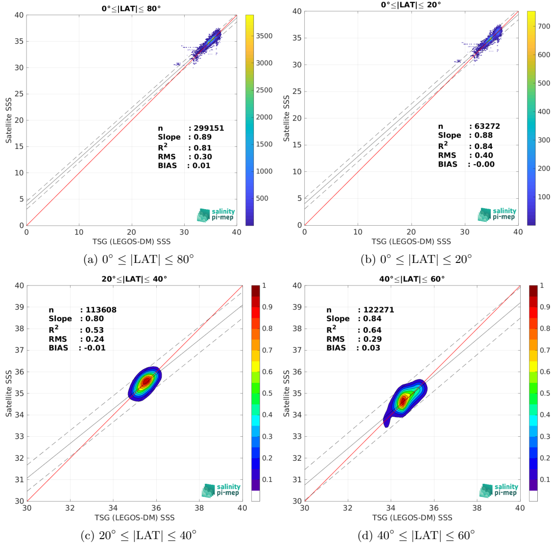
Figure 10: Contour maps of the concentration of SMOS SSS L3 v335 - Monthly - 25 km (CATDS-CPDC) SSS ( y -axis) versus TSG (LEGOS-DM) SSS ( x -axis) at match-up pairs for different latitude bands. For each plot, the red line shows x=y . The black thin and dashed lines indicate a linear fit through the data cloud and the \pm 95\% confidence levels, respectively. The number match-up pairs n , the slope and R^2 coefficient of the linear fit, the root mean square (RMS) and the mean bias between satellite and in situ data are indicated for each latitude band in each plots.
