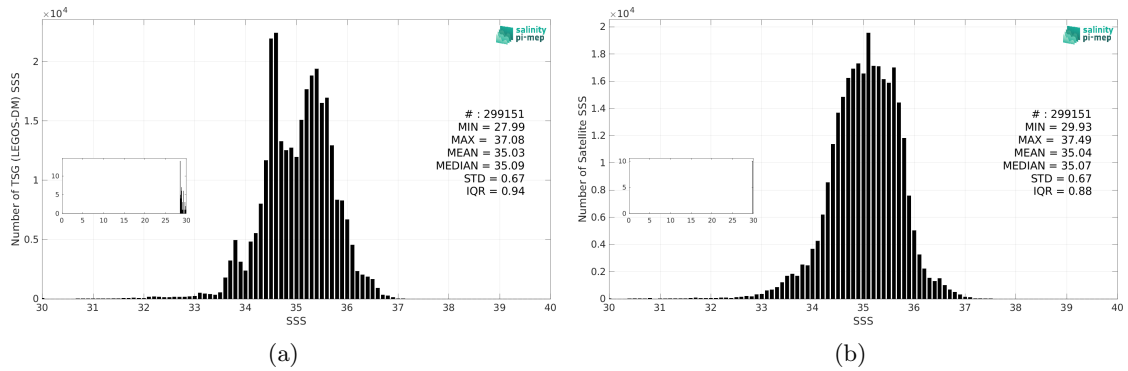
Figure 3: Histograms of SSS from TSG (LEGOS-DM) (a) and SMOS SSS L3 v335 - Monthly - 25 km (CATDS-CPDC) (b) considering all match-up pairs per bins of 0.1 over the Indian Ocean Pi-MEP region and for the full satellite product period.
