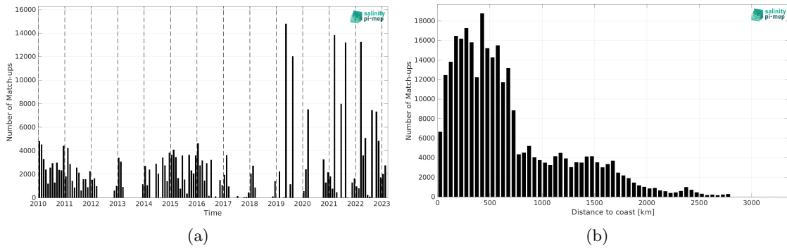
Figure 2: Number of match-ups between TSG (LEGOS-DM) and SMOS SSS L3 v335 - Monthly - 25 km (CATDS-CPDC) SSS as a function of time (a) and as function of the distance to coast (b) over the Indian Ocean Pi-MEP region and for the full satellite product period.
