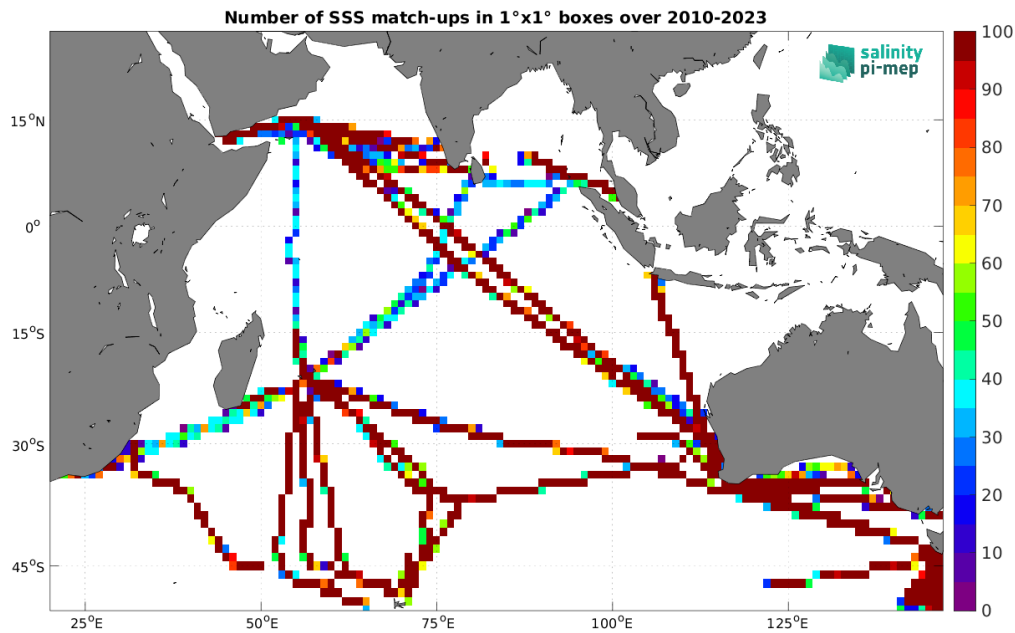
Figure 4: Number of SSS match-ups between TSG (LEGOS-DM) SSS and the SMOS SSS L3 v335 - Monthly - 25 km (CATDS-CPDC) SSS product for the Indian Ocean Pi-MEP region over 1^\circ \times 1^\circ boxes and for the full satellite product period.
