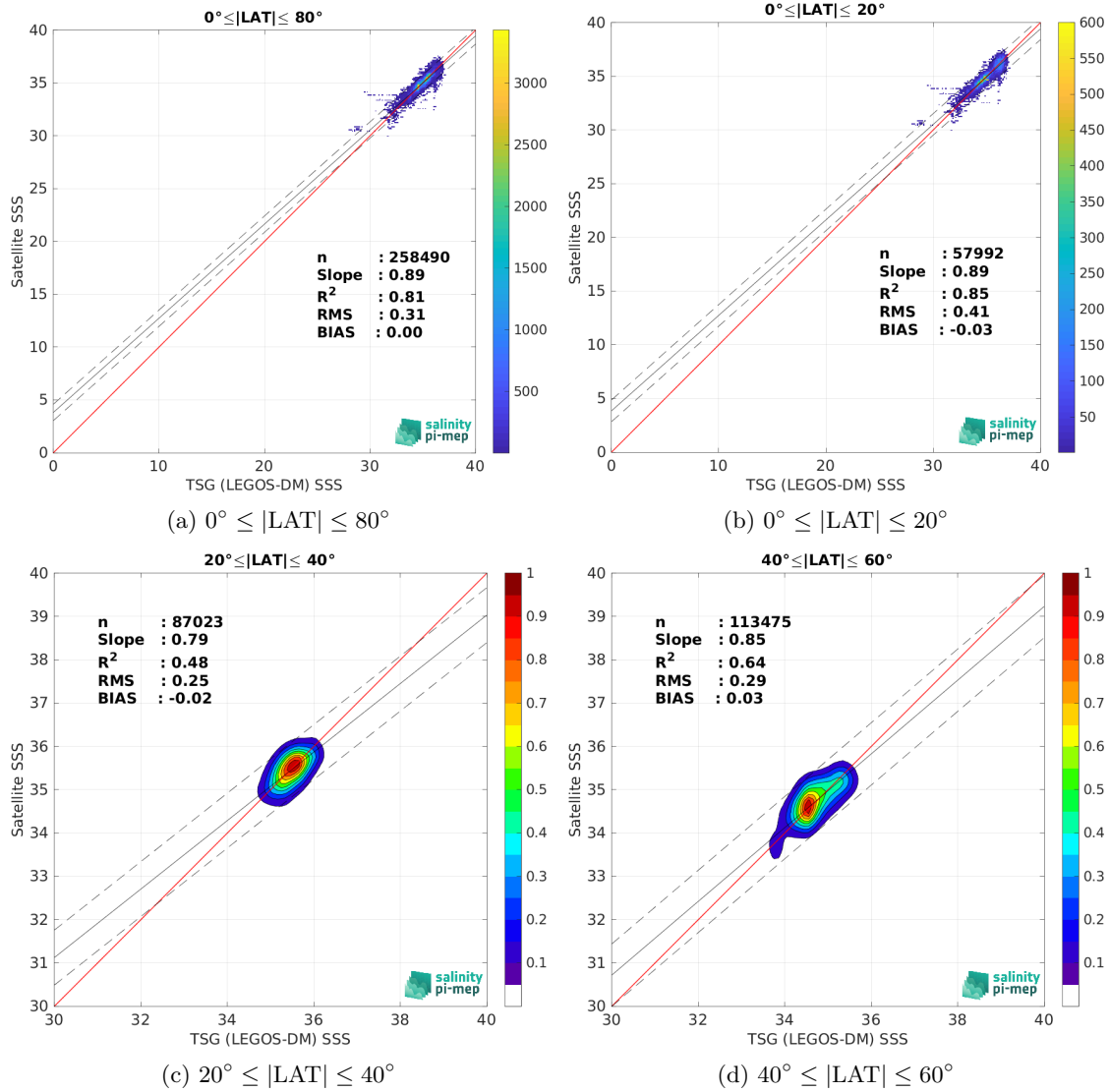
Figure 9: Contour maps of the concentration of SMOS SSS L3 v335 - Monthly - 25 km (CATDS-CPDC) SSS ( y -axis) versus TSG (LEGOS-DM) SSS ( x -axis) at match-up pairs for different latitude bands. For each plot, the red line shows x=y . The black thin and dashed lines indicate a linear fit through the data cloud and the \pm 95\% confidence levels, respectively. The number match-up pairs n , the slope and R^2 coefficient of the linear fit, the root mean square (RMS) and the mean bias between satellite and in situ data are indicated for each latitude band in each plots.
