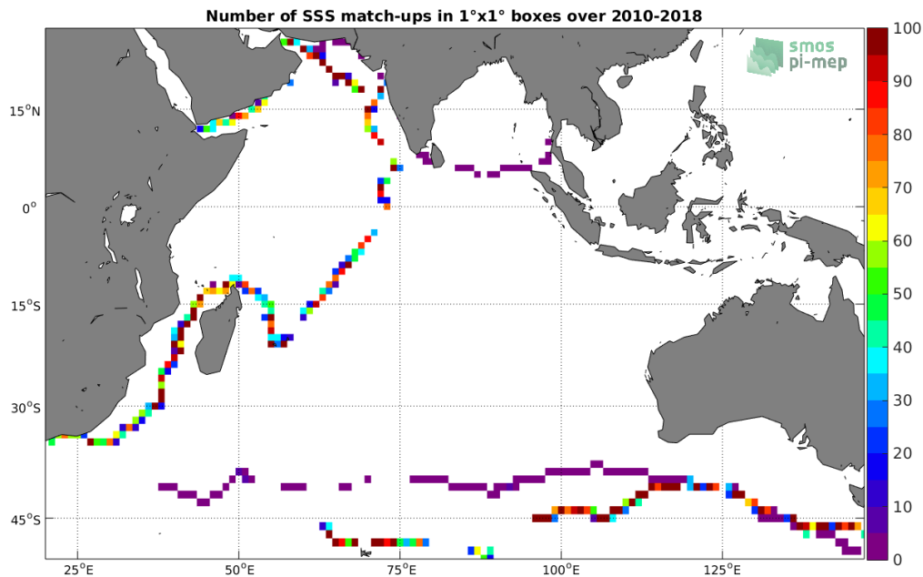
Figure 4: Number of SSS match-ups between TSG (GOSUD-Sailing-ship) SSS and the SMOS SSS L3 v335 - Monthly - 25 km (CATDS-CPDC) SSS product for the Indian Ocean Pi-MEP region over 1^\circ \times 1^\circ boxes and for the full satellite product period.
