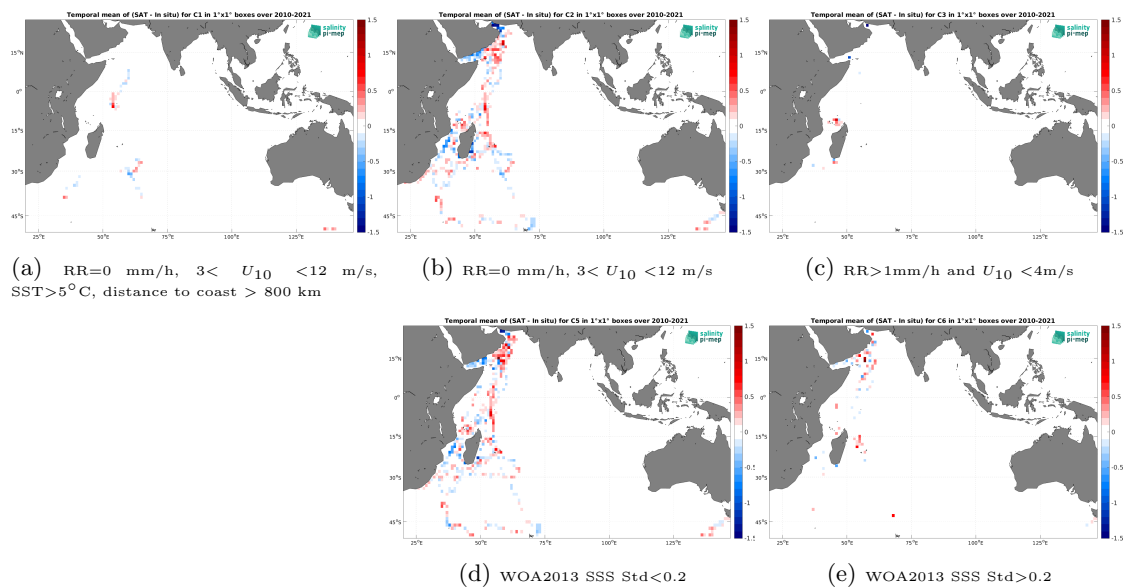
Figure 14: Temporal mean gridded over spatial boxes of size 1^\circ \times 1^\circ of \Delta SSS (SMOS SSS L3 v335 - Monthly - 25 km (CATDS-CPDC) - TSG (GOSUD-Research-vessel)) for 5 different subdatasets corresponding to:RR=0 mm/h, 3 < U_{10} < 12 m/s, SST >5^\circ C, distance to coast > 800 km (a), RR=0 mm/h, 3 < U_{10} < 12 m/s (b), RR >1 mm/h and U_{10} < 4 m/s (c), WOA2013 SSS Std <0.2 (d), WOA2013 SSS Std >0.2 (e).
