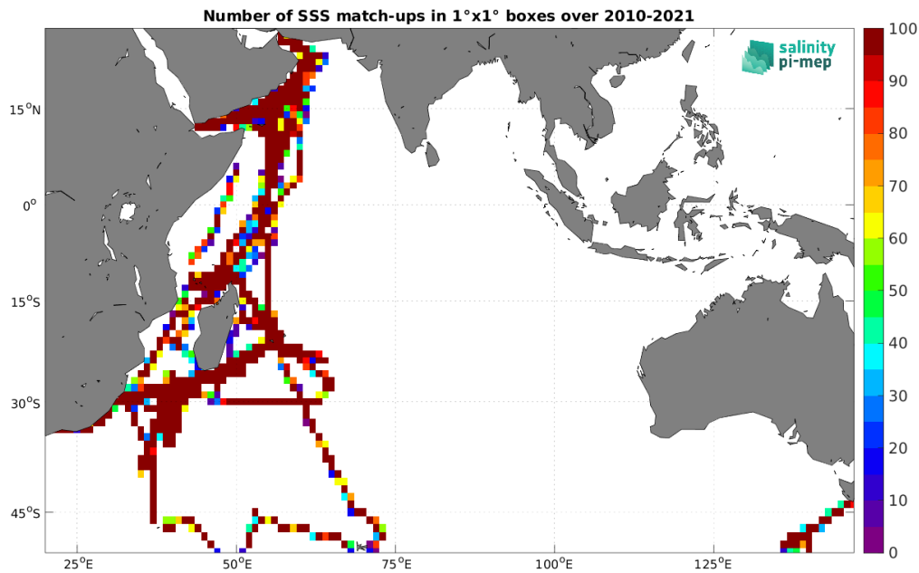
Figure 5: Number of SSS match-ups between TSG (GOSUD-Research-vessel) SSS and the SMOS SSS L3 v335 - Monthly - 25 km (CATDS-CPDC) SSS product for the Indian Ocean Pi-MEP region over 1^\circ \times 1^\circ boxes and for the full satellite product period.
