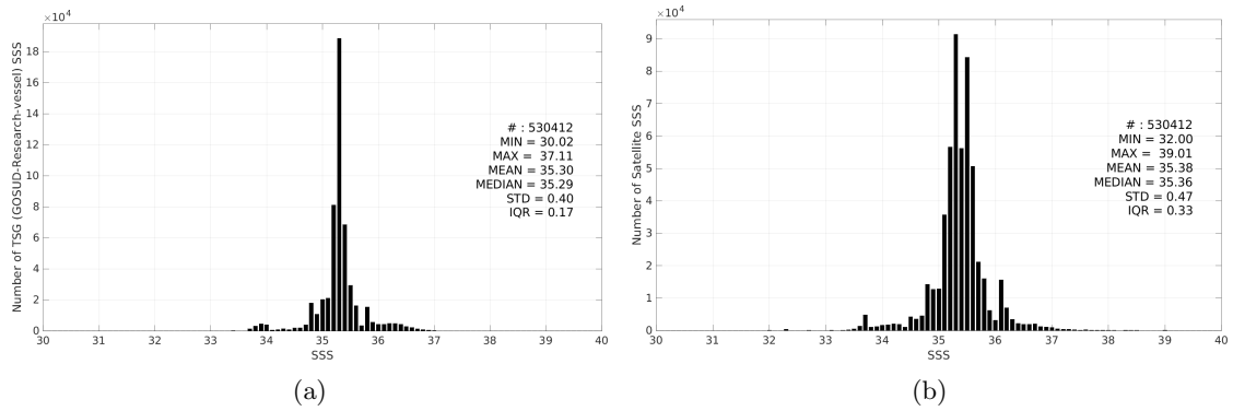
Figure 3: Histograms of SSS from TSG (GOSUD-Research-vessel) (a) and SMOS SSS L3 v335 - Monthly - 25 km (CATDS-CPDC) (b) considering all match-up pairs per bins of 0.1 over the Indian Ocean Pi-MEP region and for the full satellite product period.
