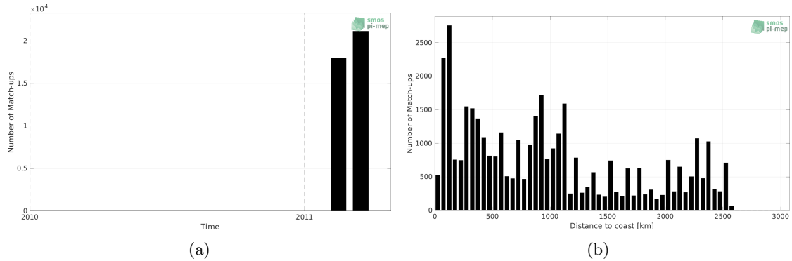
Figure 1: Number of match-ups between TSG (CSIC-UTM) and SMOS SSS L3 v335 - Monthly - 25 km (CATDS-CPDC) SSS as a function of time (a) and as function of the distance to coast (b) over the Indian Ocean Pi-MEP region and for the full satellite product period.
