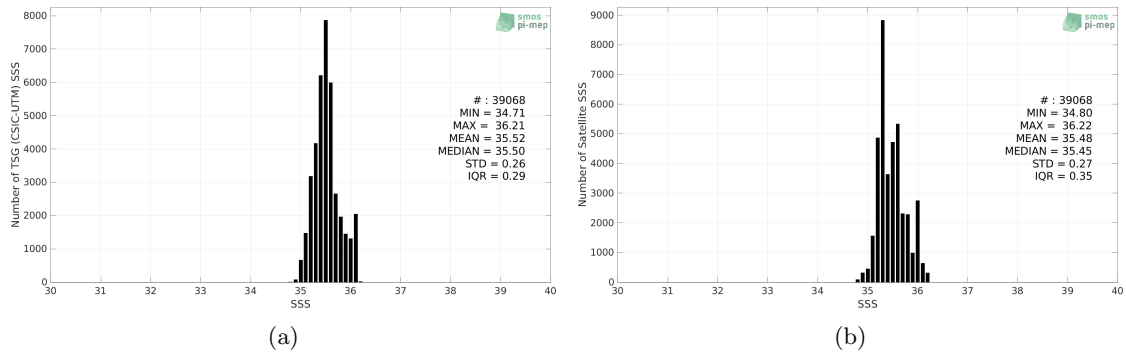
Figure 2: Histograms of SSS from TSG (CSIC-UTM) (a) and SMOS SSS L3 v335 - Monthly - 25 km (CATDS-CPDC) (b) considering all match-up pairs per bins of 0.1 over the Indian Ocean Pi-MEP region and for the full satellite product period.
