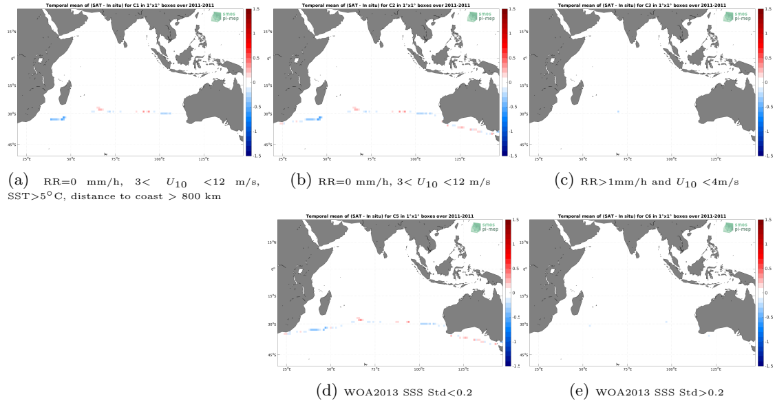
Figure 12: Temporal mean gridded over spatial boxes of size 1^{\circ}\times 1^{\circ} of \Delta\text{SSS} (SMOS SSS L3 v335 - Monthly - 25 km (CATDS-CPDC) - TSG (CSIC-UTM)) for 5 different subdatasets corresponding to:RR=0 mm/h, 3 < U_{10} < 12 m/s, SST >5^{\circ}\text{C} , distance to coast > 800 km (a), RR=0 mm/h, 3 < U_{10} < 12 m/s (b), RR >1 mm/h and U_{10} < 4 m/s (c), WOA2013 SSS Std <0.2 (d), WOA2013 SSS Std >0.2 (e).
