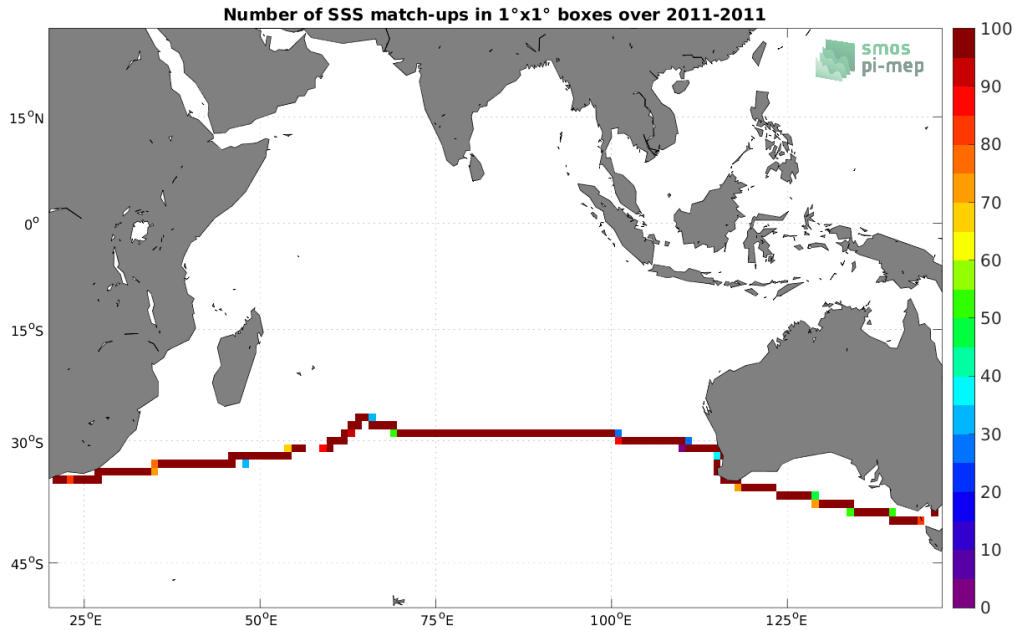
Figure 4: Number of SSS match-ups between TSG (CSIC-UTM) SSS and the SMOS SSS L3 v335 - Monthly - 25 km (CATDS-CPDC) SSS product for the Indian Ocean Pi-MEP region over 1^\circ \times 1^\circ boxes and for the full satellite product period.
