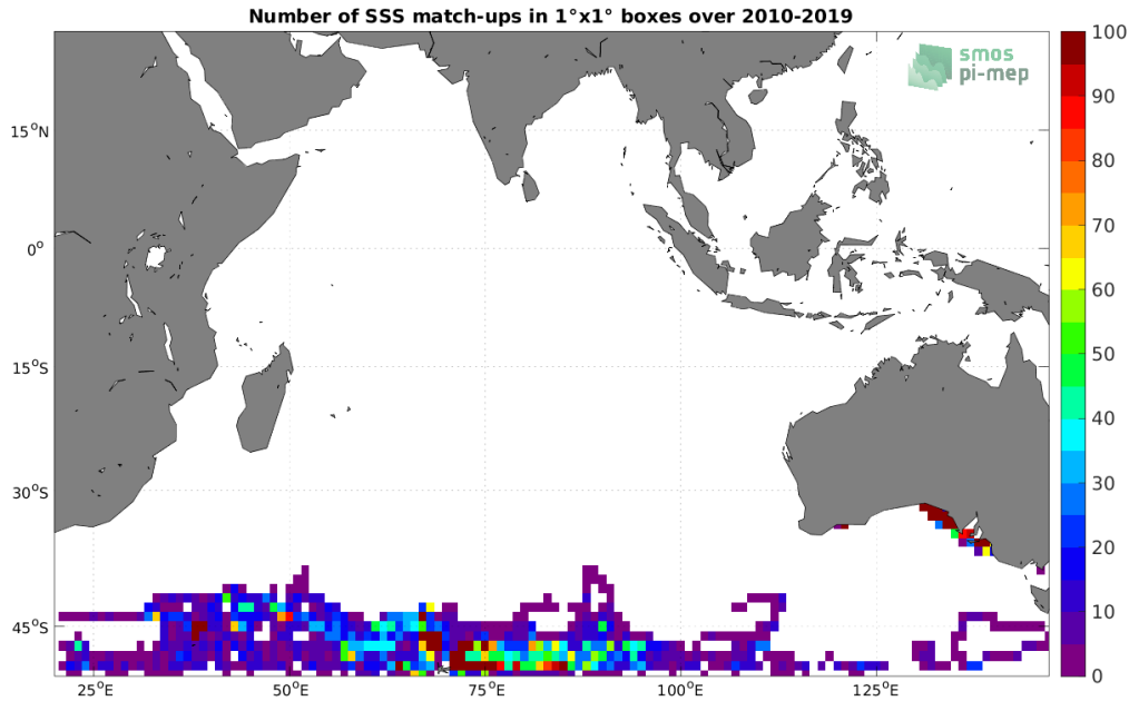
Figure 4: Number of SSS match-ups between Marine mammals SSS and the SMOS SSS L3 v335 - Monthly - 25 km (CATDS-CPDC) SSS product for the Indian Ocean Pi-MEP region over 1^\circ \times 1^\circ boxes and for the full satellite product period.
