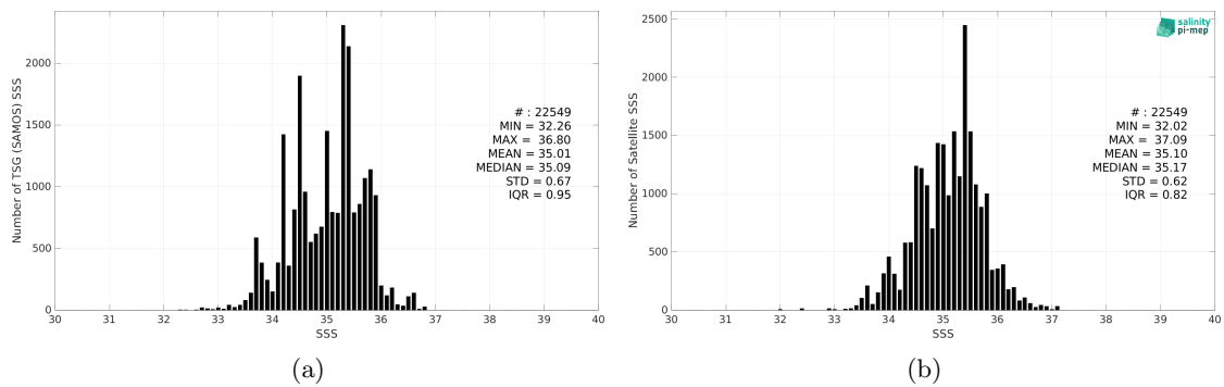
Figure 2: Histograms of SSS from TSG (SAMOS) (a) and SMOS SSS L3 v335 - 10 Days - 25 km (CATDS-CPDC) (b) considering all match-up pairs per bins of 0.1 over the Indian Ocean Pi-MEP region and for the full satellite product period.
