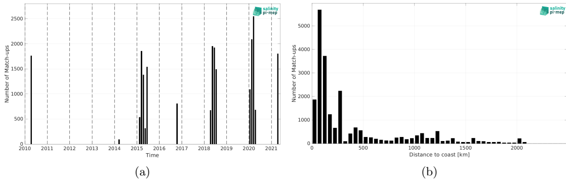
Figure 1: Number of match-ups between TSG (SAMOS) and SMOS SSS L3 v335 - 10 Days - 25 km (CATDS-CPDC) SSS as a function of time (a) and as function of the distance to coast (b) over the Indian Ocean Pi-MEP region and for the full satellite product period.
