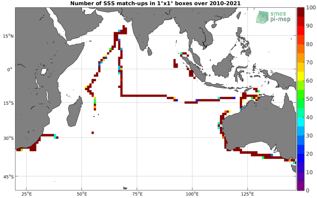
Figure 4: Number of SSS match-ups between TSG (SAMOS) SSS and the SMOS SSS L3 v335 - 10 Days - 25 km (CATDS-CPDC) SSS product for the Indian Ocean Pi-MEP region over 1^\circ \times 1^\circ boxes and for the full satellite product period.
