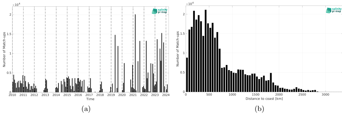
Figure 2: Number of match-ups between TSG (LEGOS-DM) and SMOS SSS L3 v335 - 10 Days - 25 km (CATDS-CPDC) SSS as a function of time (a) and as function of the distance to coast (b) over the Indian Ocean Pi-MEP region and for the full satellite product period.
