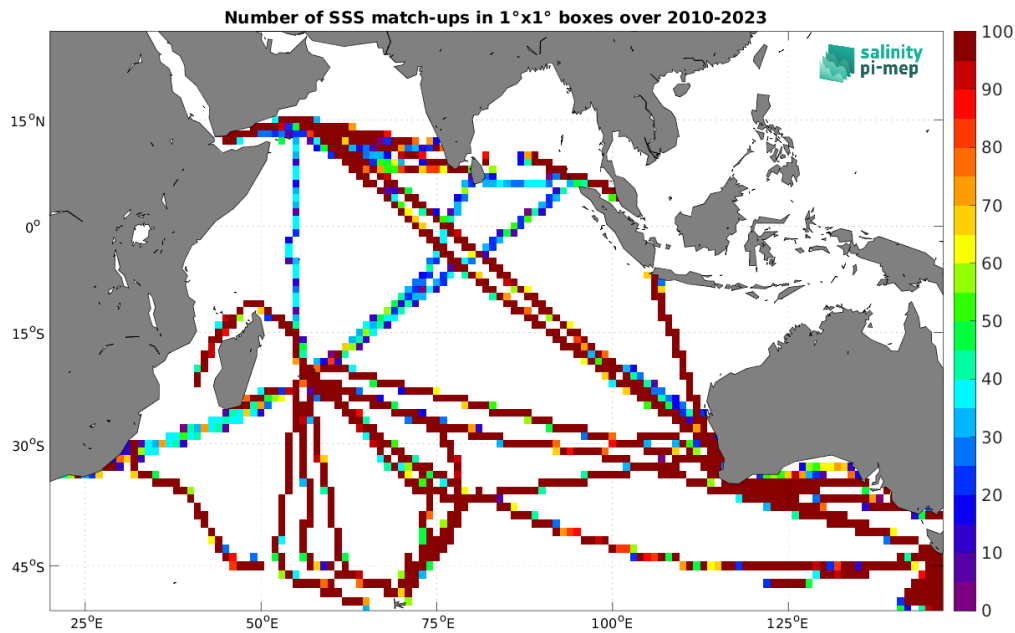
Figure 5: Number of SSS match-ups between TSG (LEGOS-DM) SSS and the SMOS SSS L3 v335 - 10 Days - 25 km (CATDS-CPDC) SSS product for the Indian Ocean Pi-MEP region over 1^\circ \times 1^\circ boxes and for the full satellite product period.
