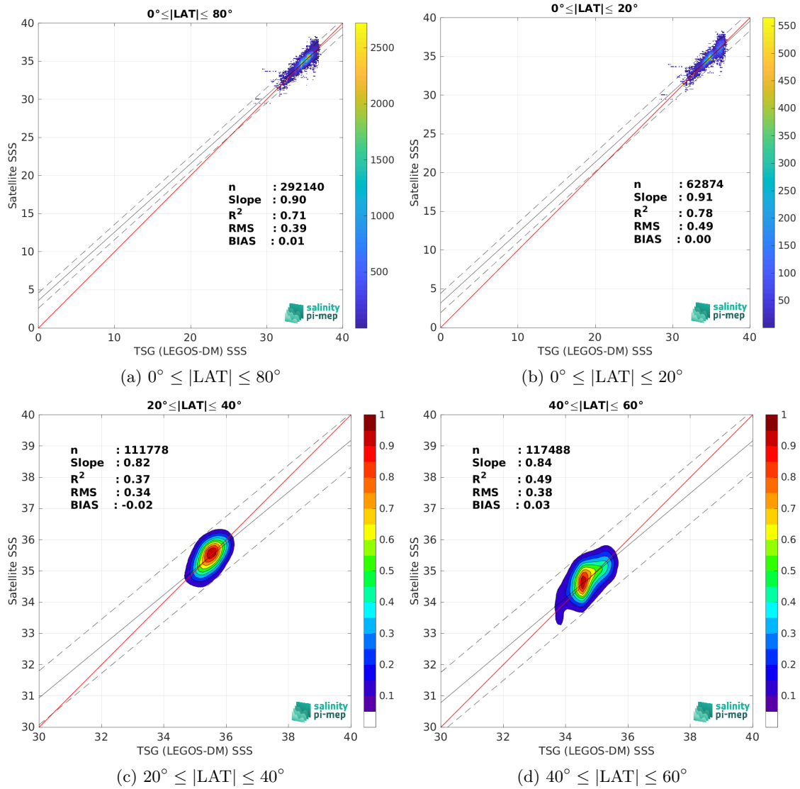
Figure 10: Contour maps of the concentration of SMOS SSS L3 v335 - 10 Days - 25 km (CATDS-CPDC) SSS ( y -axis) versus TSG (LEGOS-DM) SSS ( x -axis) at match-up pairs for different latitude bands. For each plot, the red line shows x=y . The black thin and dashed lines indicate a linear fit through the data cloud and the \pm 95\% confidence levels, respectively. The number match-up pairs n , the slope and R^2 coefficient of the linear fit, the root mean square (RMS) and the mean bias between satellite and in situ data are indicated for each latitude band in each plots.
