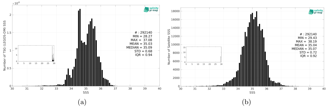
Figure 3: Histograms of SSS from TSG (LEGOS-DM) (a) and SMOS SSS L3 v335 - 10 Days - 25 km (CATDS-CPDC) (b) considering all match-up pairs per bins of 0.1 over the Indian Ocean Pi-MEP region and for the full satellite product period.
