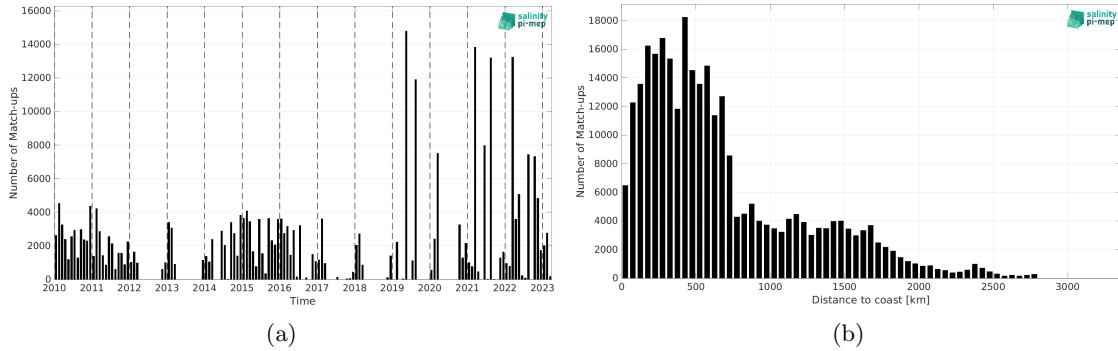
Figure 2: Number of match-ups between TSG (LEGOS-DM) and SMOS SSS L3 v335 - 10 Days - 25 km (CATDS-CPDC) SSS as a function of time (a) and as function of the distance to coast (b) over the Indian Ocean Pi-MEP region and for the full satellite product period.
