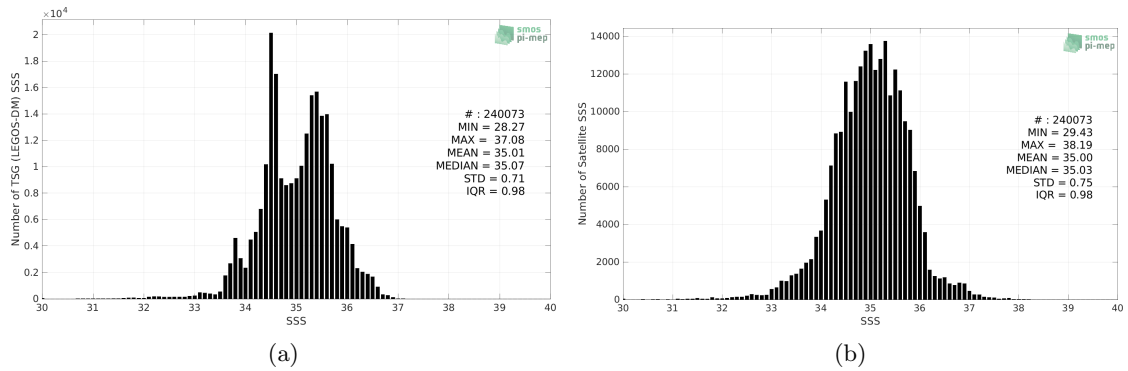
Figure 2: Histograms of SSS from TSG (LEGOS-DM) (a) and SMOS SSS L3 v335 - 10 Days - 25 km (CATDS-CPDC) (b) considering all match-up pairs per bins of 0.1 over the Indian Ocean Pi-MEP region and for the full satellite product period.
