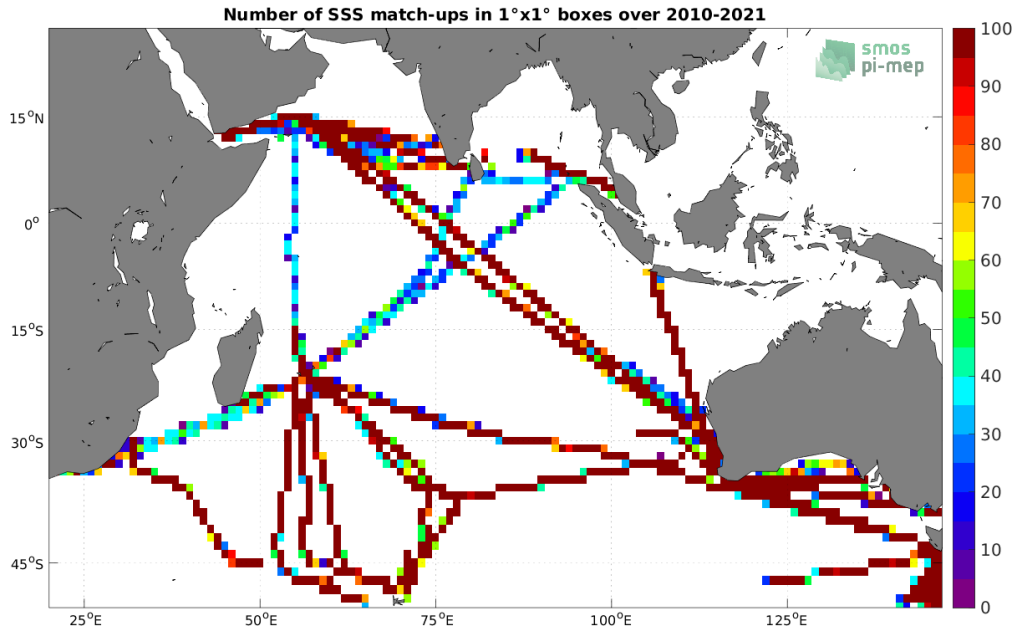
Figure 4: Number of SSS match-ups between TSG (LEGOS-DM) SSS and the SMOS SSS L3 v335 - 10 Days - 25 km (CATDS-CPDC) SSS product for the Indian Ocean Pi-MEP region over 1^\circ \times 1^\circ boxes and for the full satellite product period.
