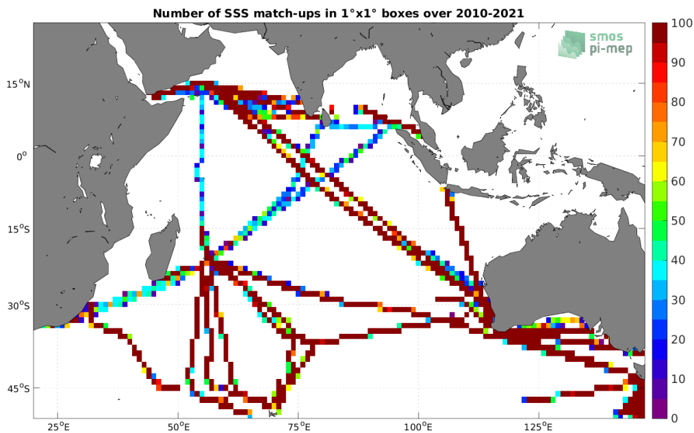
Figure 4: Number of SSS match-ups between TSG (LEGOS-DM) SSS and the SMOS SSS L3 v335 - 10 Days - 25 km (CATDS-CPDC) SSS product for the Indian Ocean Pi-MEP region over 1^\circ \times 1^\circ boxes and for the full satellite product period.
