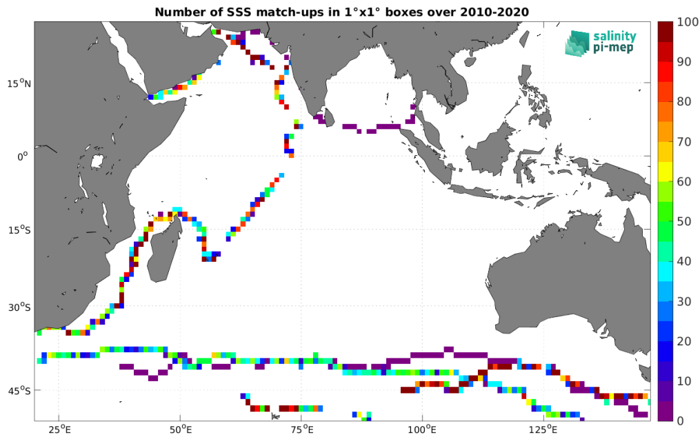
Figure 5: Number of SSS match-ups between TSG (GOSUD-Sailing-ship) SSS and the SMOS SSS L3 v335 - 10 Days - 25 km (CATDS-CPDC) SSS product for the Indian Ocean Pi-MEP region over 1^\circ \times 1^\circ boxes and for the full satellite product period.
