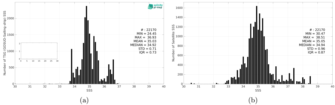
Figure 3: Histograms of SSS from TSG (GOSUD-Sailing-ship) (a) and SMOS SSS L3 v335 - 10 Days - 25 km (CATDS-CPDC) (b) considering all match-up pairs per bins of 0.1 over the Indian Ocean Pi-MEP region and for the full satellite product period.
