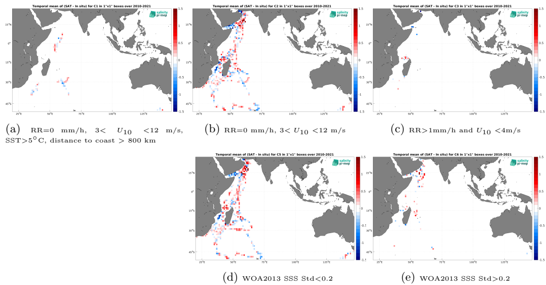
Figure 14: Temporal mean gridded over spatial boxes of size 1^\circ \times 1^\circ of \Delta SSS (SMOS SSS L3 v335 - 10 Days - 25 km (CATDS-CPDC) - TSG (GOSUD-Research-vessel)) for 5 different subdatasets corresponding to:RR=0 mm/h, 3 < U_{10} < 12 m/s, SST >5^\circ C, distance to coast > 800 km (a), RR=0 mm/h, 3 < U_{10} < 12 m/s (b), RR >1 mm/h and U_{10} < 4 m/s (c), WOA2013 SSS Std <0.2 (d), WOA2013 SSS Std >0.2 (e).
