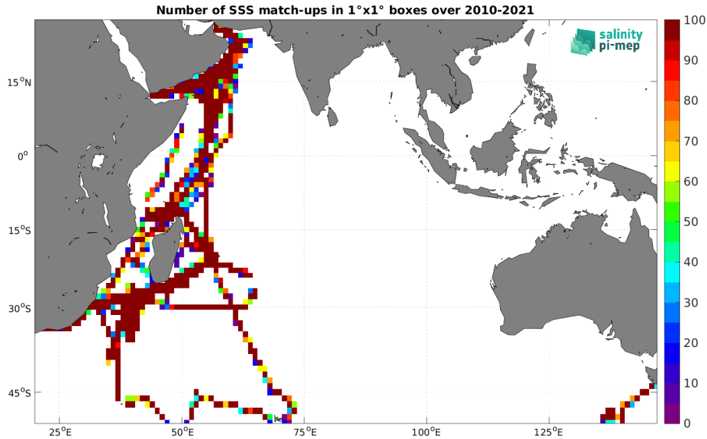
Figure 5: Number of SSS match-ups between TSG (GOSUD-Research-vessel) SSS and the SMOS SSS L3 v335 - 10 Days - 25 km (CATDS-CPDC) SSS product for the Indian Ocean Pi-MEP region over 1^\circ \times 1^\circ boxes and for the full satellite product period.
