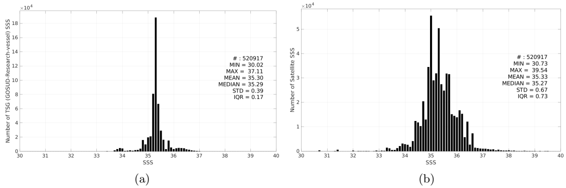
Figure 3: Histograms of SSS from TSG (GOSUD-Research-vessel) (a) and SMOS SSS L3 v335 - 10 Days - 25 km (CATDS-CPDC) (b) considering all match-up pairs per bins of 0.1 over the Indian Ocean Pi-MEP region and for the full satellite product period.
