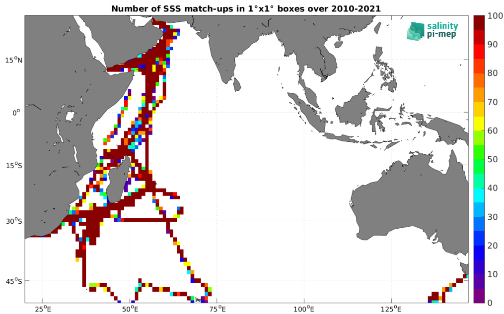
Figure 4: Number of SSS match-ups between TSG (GOSUD-Research-vessel) SSS and the SMOS SSS L3 v335 - 10 Days - 25 km (CATDS-CPDC) SSS product for the Indian Ocean Pi-MEP region over 1^\circ \times 1^\circ boxes and for the full satellite product period.
