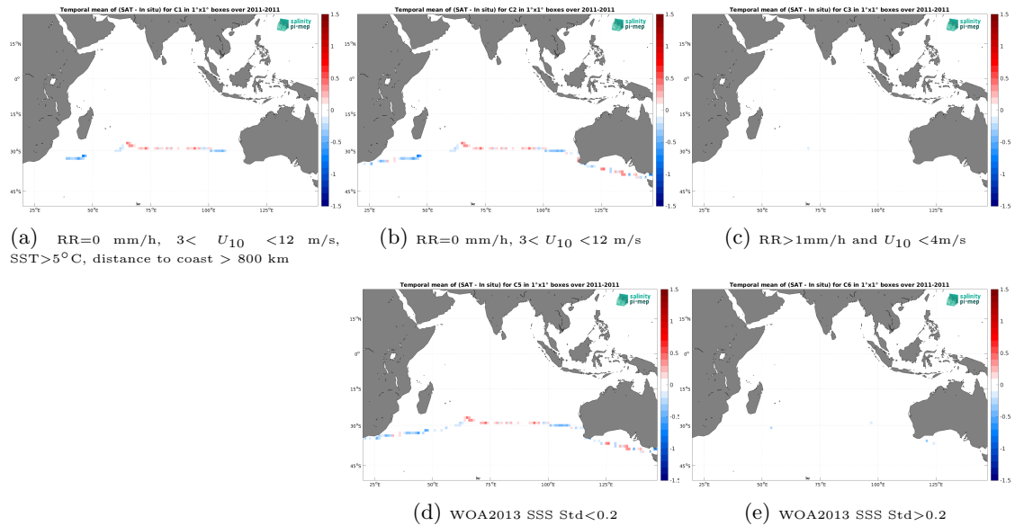
Figure 12: Temporal mean gridded over spatial boxes of size 1^{\circ}\times 1^{\circ} of \Delta\text{SSS} (SMOS SSS L3 v335 - 10 Days - 25 km (CATDS-CPDC) - TSG (CSIC-UTM)) for 5 different subdatasets corresponding to:RR=0 mm/h, 3 < U_{10} < 12 m/s, SST >5^{\circ}\text{C} , distance to coast > 800 km (a), RR=0 mm/h, 3 < U_{10} < 12 m/s (b), RR >1 mm/h and U_{10} < 4 m/s (c), WOA2013 SSS Std <0.2 (d), WOA2013 SSS Std >0.2 (e).
