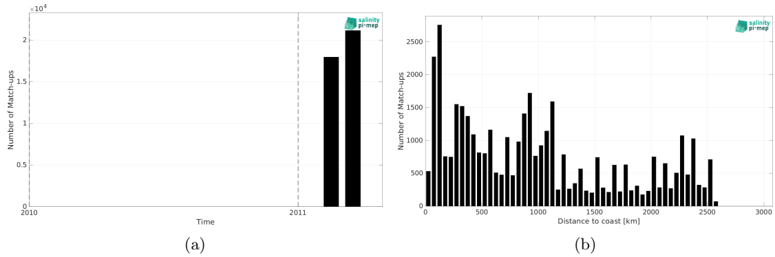
Figure 1: Number of match-ups between TSG (CSIC-UTM) and SMOS SSS L3 v335 - 10 Days - 25 km (CATDS-CPDC) SSS as a function of time (a) and as function of the distance to coast (b) over the Indian Ocean Pi-MEP region and for the full satellite product period.
