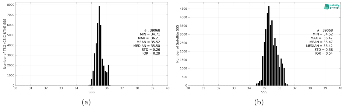
Figure 2: Histograms of SSS from TSG (CSIC-UTM) (a) and SMOS SSS L3 v335 - 10 Days - 25 km (CATDS-CPDC) (b) considering all match-up pairs per bins of 0.1 over the Indian Ocean Pi-MEP region and for the full satellite product period.
