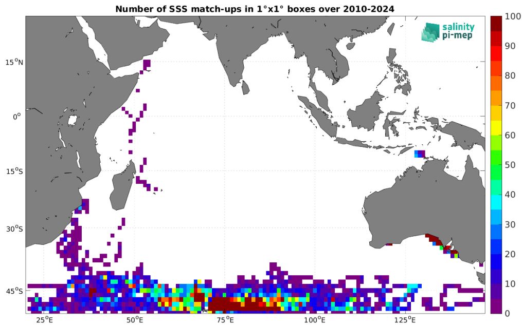
Figure 5: Number of SSS match-ups between Marine mammals SSS and the SMOS SSS L3 v335 - 10 Days - 25 km (CATDS-CPDC) SSS product for the Indian Ocean Pi-MEP region over 1^\circ \times 1^\circ boxes and for the full satellite product period.
