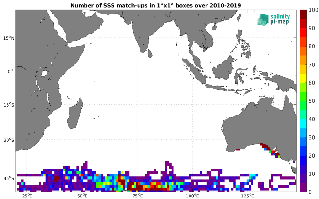
Figure 4: Number of SSS match-ups between Marine mammals SSS and the SMOS SSS L3 v335 - 10 Days - 25 km (CATDS-CPDC) SSS product for the Indian Ocean Pi-MEP region over 1^\circ \times 1^\circ boxes and for the full satellite product period.
