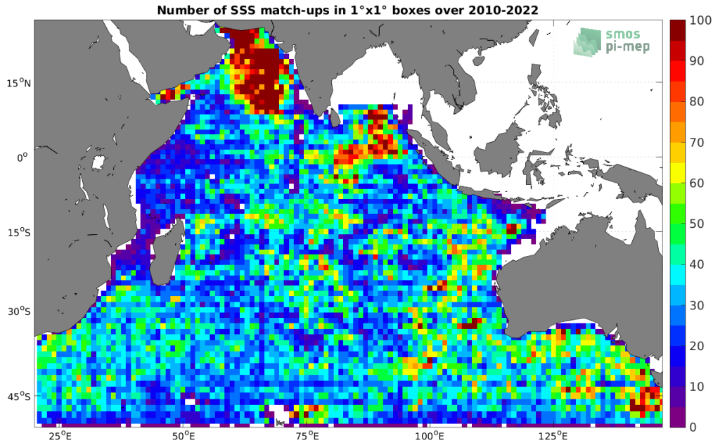
Figure 4: Number of SSS match-ups between Argo SSS and the SMOS SSS L3 v335 - 10 Days - 25 km (CATDS-CPDC) SSS product for the Indian Ocean Pi-MEP region over 1^{\circ} \times 1^{\circ} boxes and for the full satellite product period.
