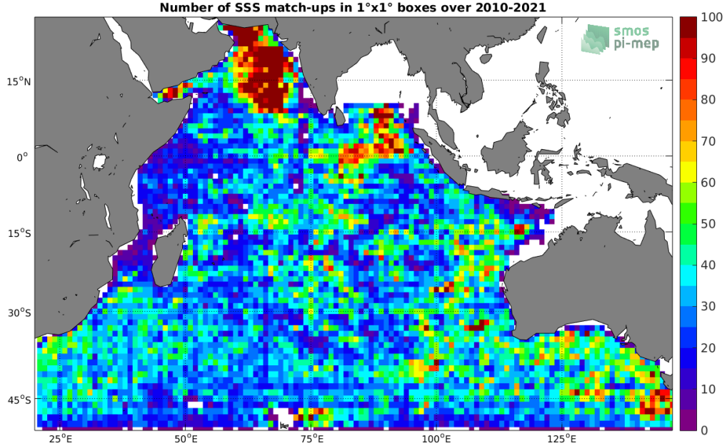
Figure 4: Number of SSS match-ups between Argo SSS and the SMOS SSS L3 v335 - 10 Days - 25 km (CATDS-CPDC) SSS product for the Indian Ocean Pi-MEP region over 1^\circ \times 1^\circ boxes and for the full satellite product period.
