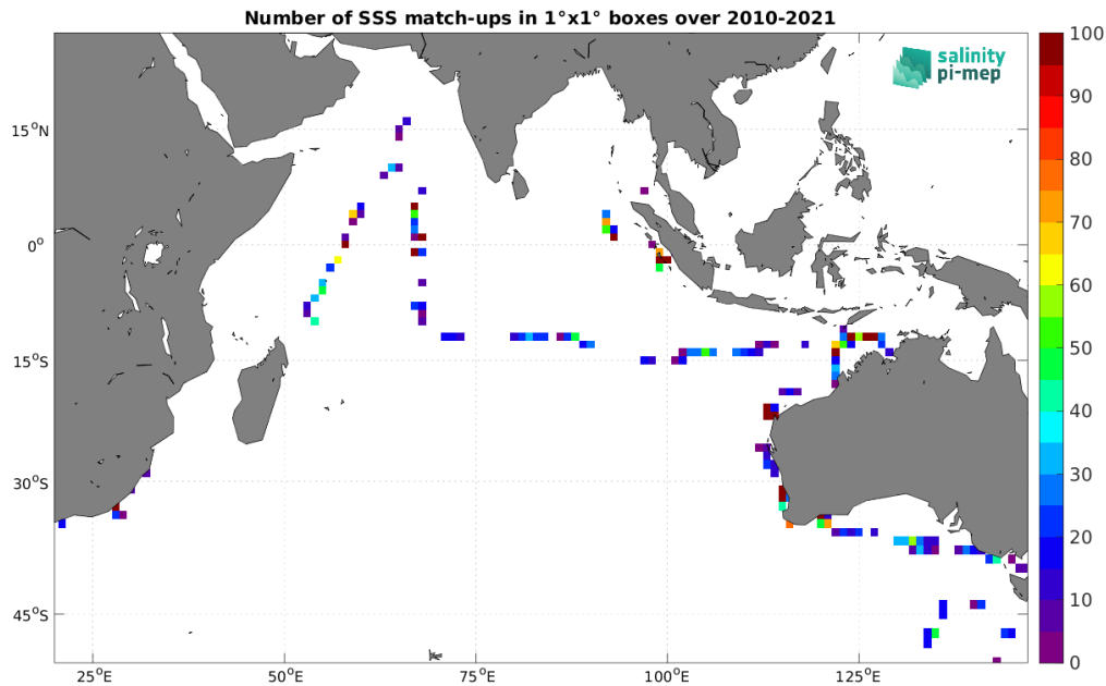
Figure 5: Number of SSS match-ups between TSG (SAMOS) SSS and the SMOS SSS L2Q v333 - 0.25 Deg (CATDS-CPDC) SSS product for the Indian Ocean Pi-MEP region over 1^\circ \times 1^\circ boxes and for the full satellite product period.
