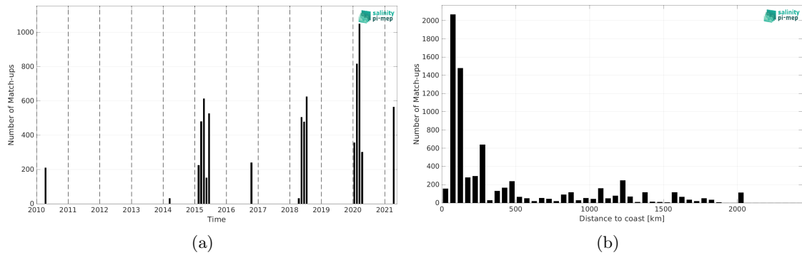
Figure 2: Number of match-ups between TSG (SAMOS) and SMOS SSS L2Q v333 - 0.25 Deg (CATDS-CPDC) SSS as a function of time (a) and as function of the distance to coast (b) over the Indian Ocean Pi-MEP region and for the full satellite product period.
