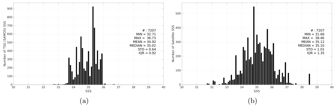
Figure 3: Histograms of SSS from TSG (SAMOS) (a) and SMOS SSS L2Q v333 - 0.25 Deg (CATDS-CPDC) (b) considering all match-up pairs per bins of 0.1 over the Indian Ocean Pi-MEP region and for the full satellite product period.
