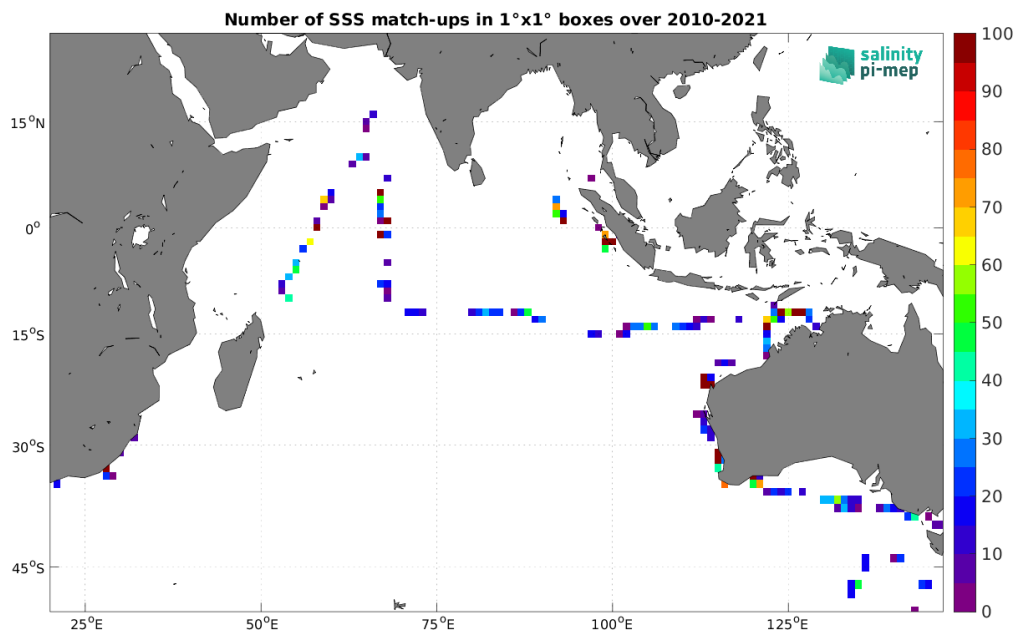
Figure 5: Number of SSS match-ups between TSG (SAMOS) SSS and the SMOS SSS L2Q v333 - 0.25 Deg (CATDS-CPDC) SSS product for the Indian Ocean Pi-MEP region over 1^\circ \times 1^\circ boxes and for the full satellite product period.
